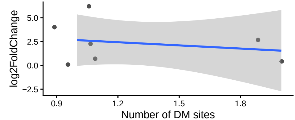
M3: Correlation # DM sites vs expr (direct
