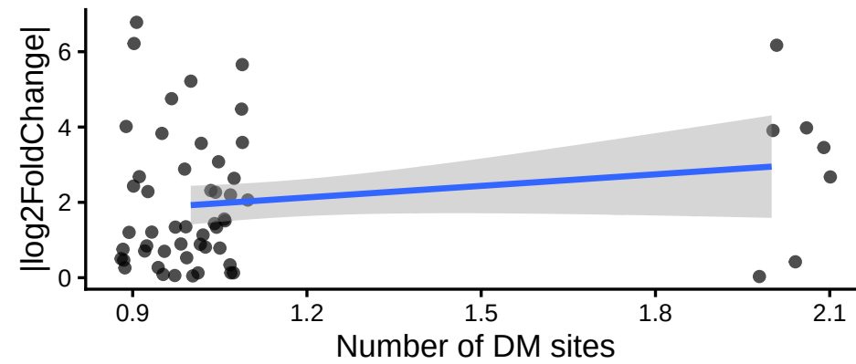
M2: Correlation # DM sites vs expr (direct1
