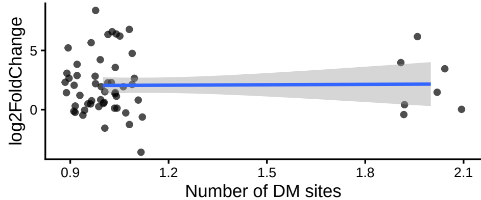
M4: Correlation # DM sites vs expr (magn
