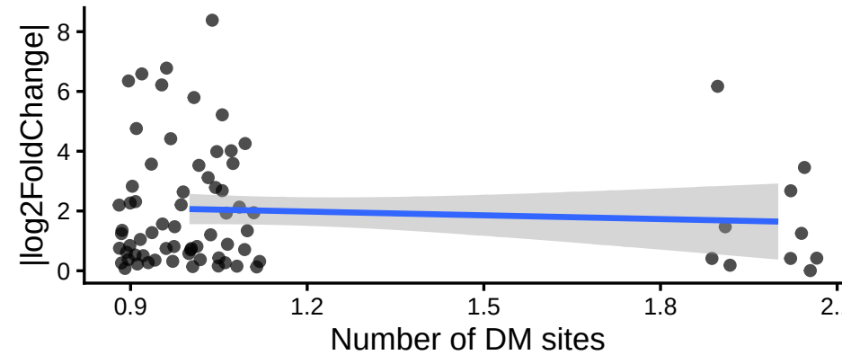
M5: Correlation # DM sites vs expr (direction)
