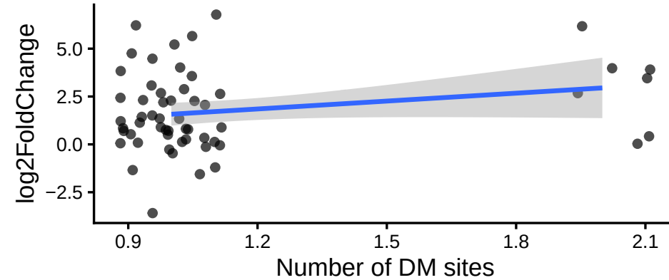
M5: Correlation # DM sites vs expr (magnitude)
