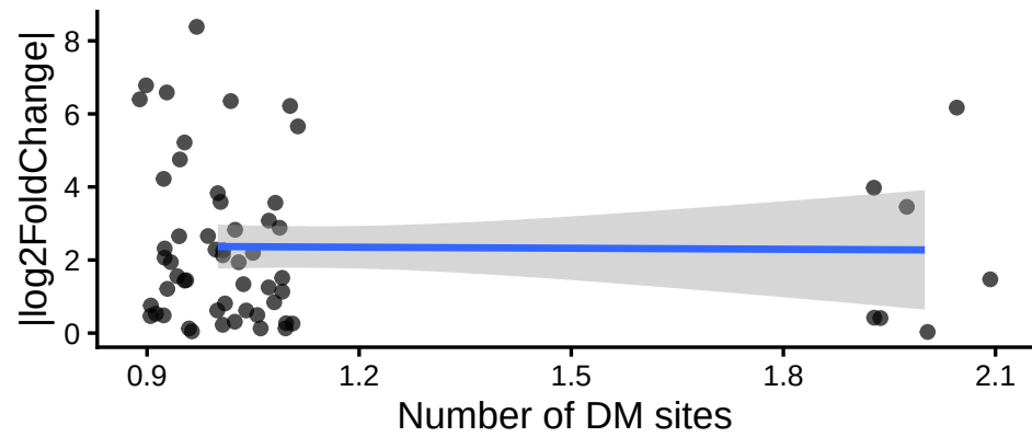
M1: Correlation # DM sites vs expr (directio
