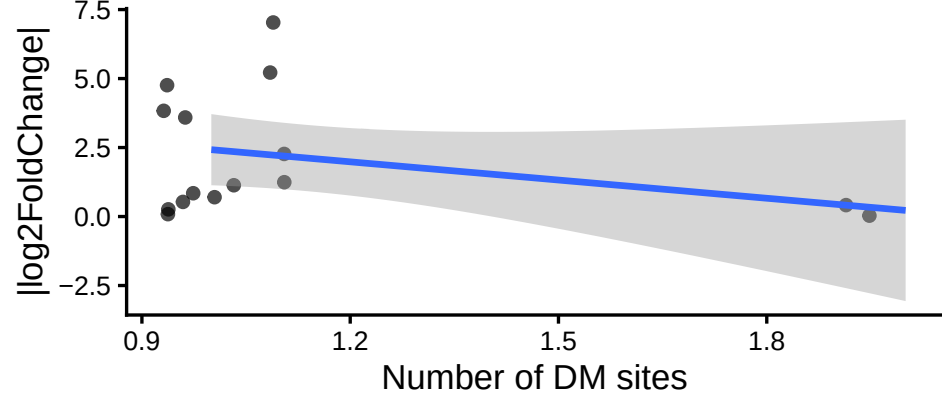
M4: Correlation # DM sites vs expr (direct1
