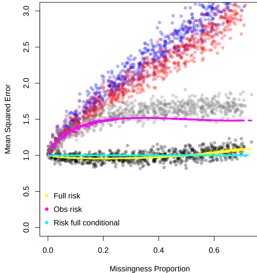
Bayes optimal forecaster
