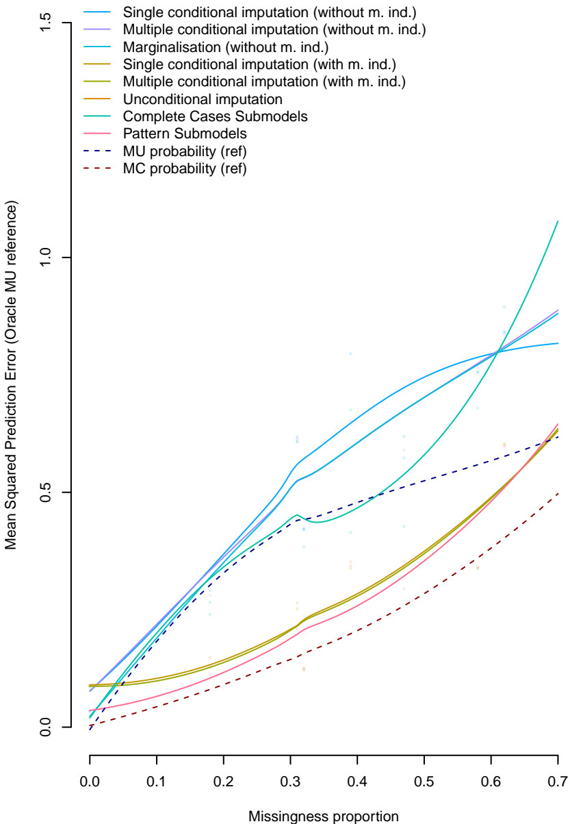
Model 3, All cases
