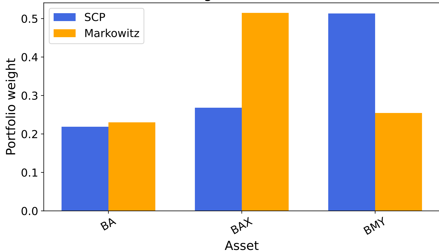
Portfolio weights: SCP vs Markowitz
