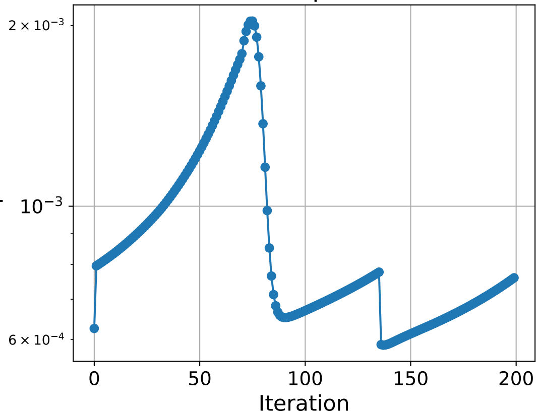
SCP: Step norm
