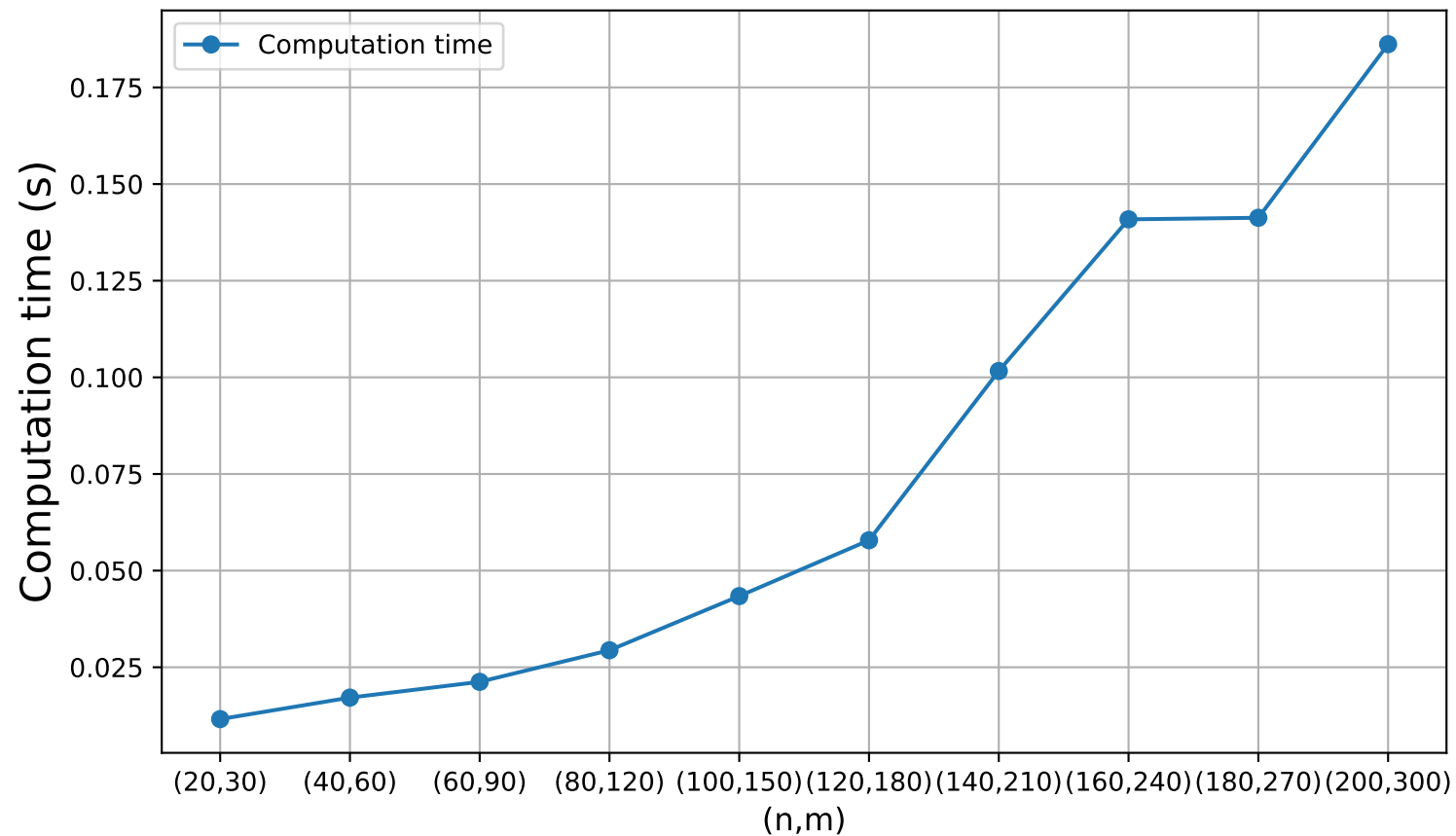
CVXPY solve time as a function of n and m
