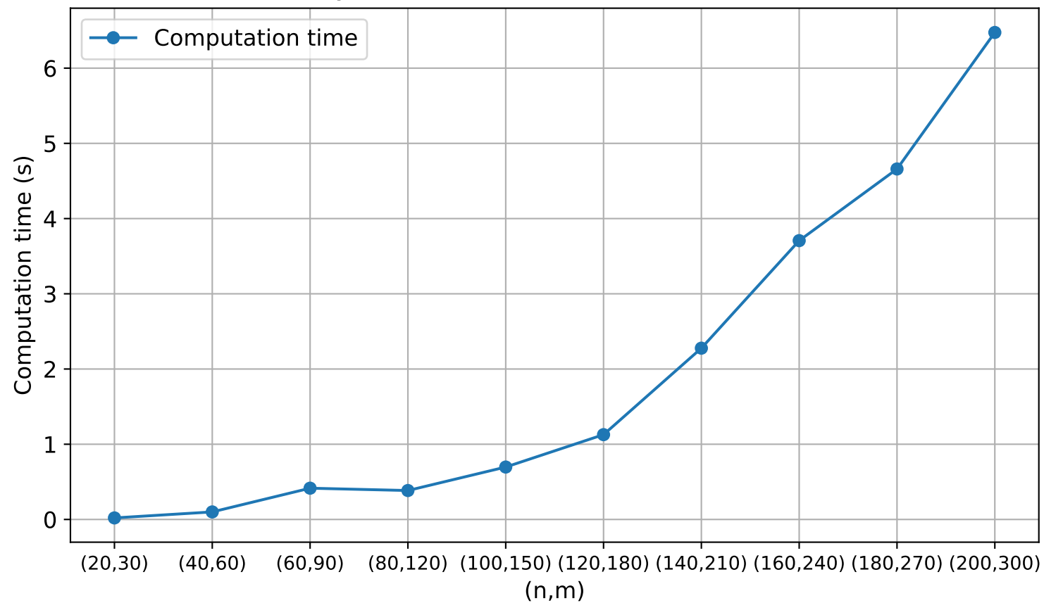
SLSQP solve time as a function of n and m
