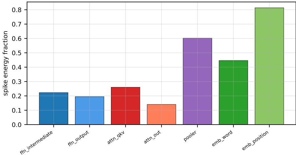
Signal energy above MP bulk (real)
