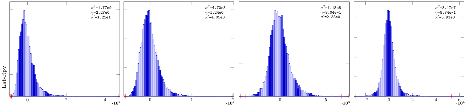
Gaussian-32-Lat-Rpv-10
