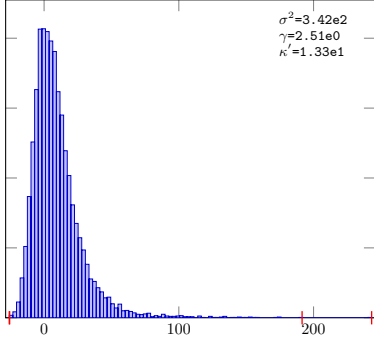
Gaussian-16-Sob-LMS-RDS-10
