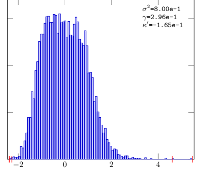
Gaussian-16-Sob-RDSB-16
