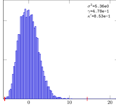
Gaussian-16-Sob-RDSB-14
