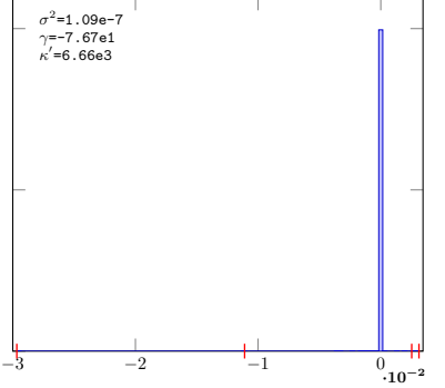
Gaussian-2-Lat-RpvRS-16
