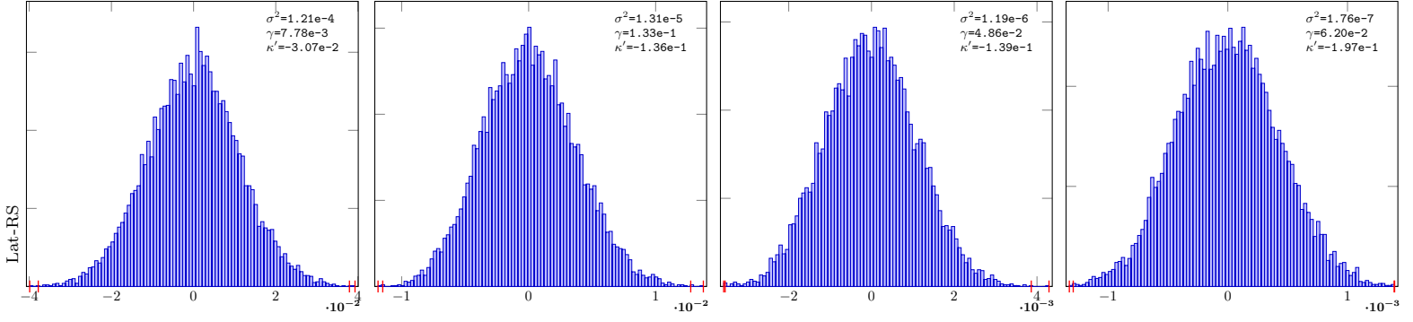
Gaussian-4-Lat-RSB-10
