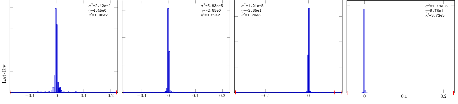
Gaussian-2-Lat-Rpv-10
