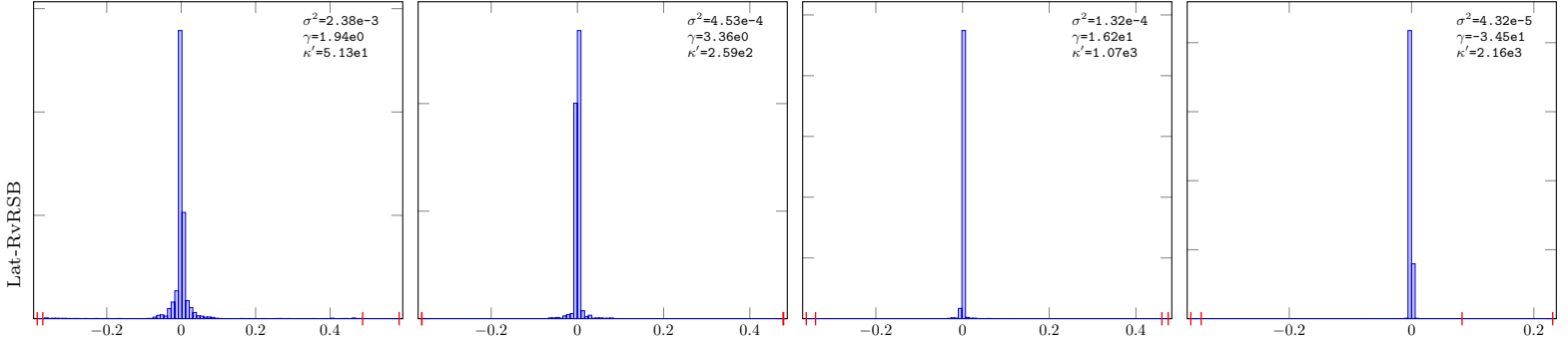
Gaussian-4-Lat-RpvRS-10
