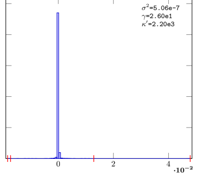
Gaussian-2-Lat-RvRSB-16
