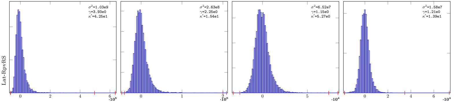
Gaussian-32-Lat-RpvRSB-10
