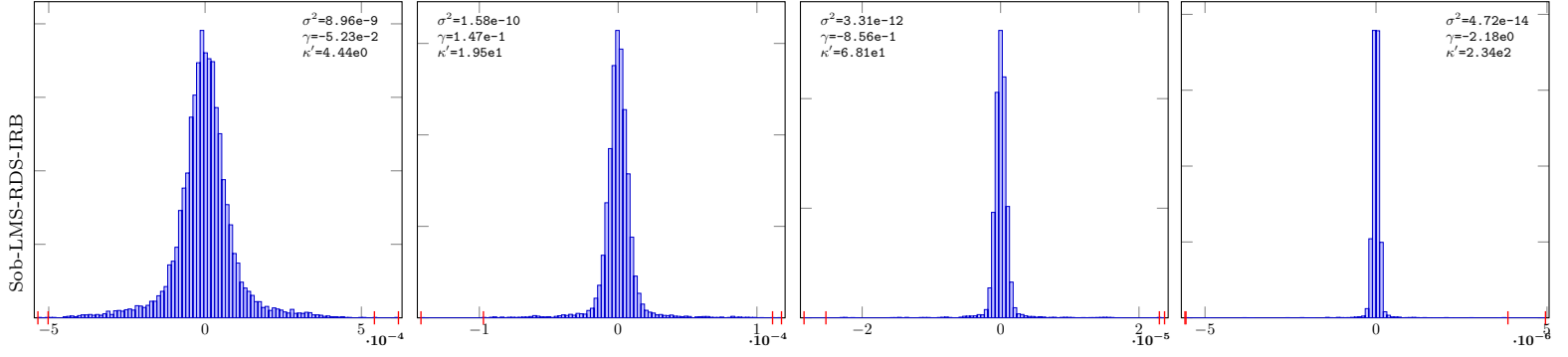
Gaussian-2-Sob-NUS-10
