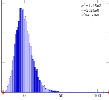
Gaussian-16-Sob-RDSB-10
