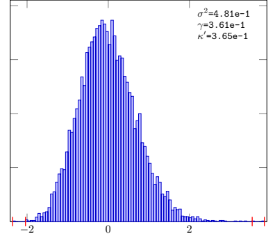
Gaussian-16-Sob-LMS-16
