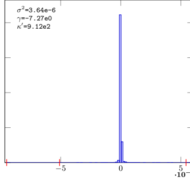
Gaussian-2-Lat-RpvRSB-14
