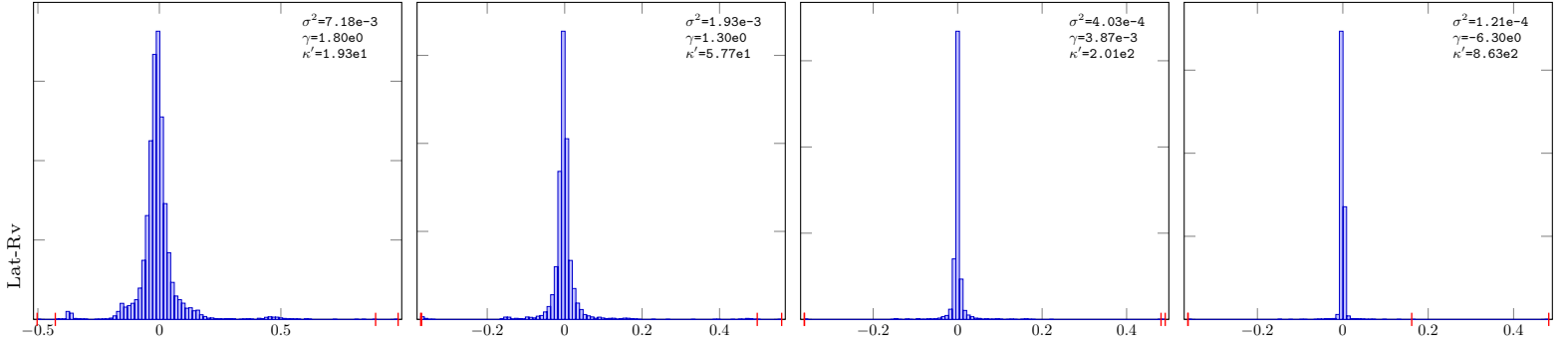
Gaussian-4-Lat-Rpv-10
