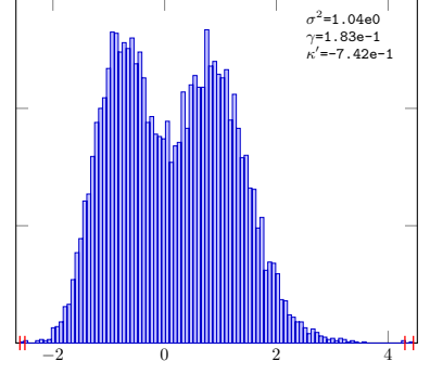
Gaussian-16-Sob-LMS-RDS-16
