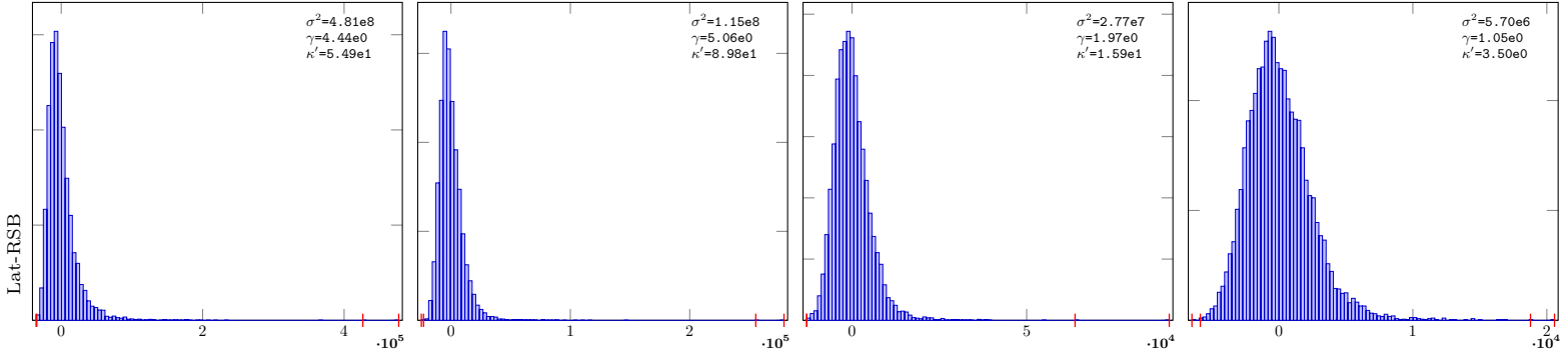
Gaussian-32-Lat-Rv-10
