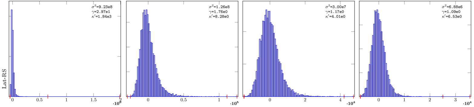
Gaussian-32-Lat-RSB-10
