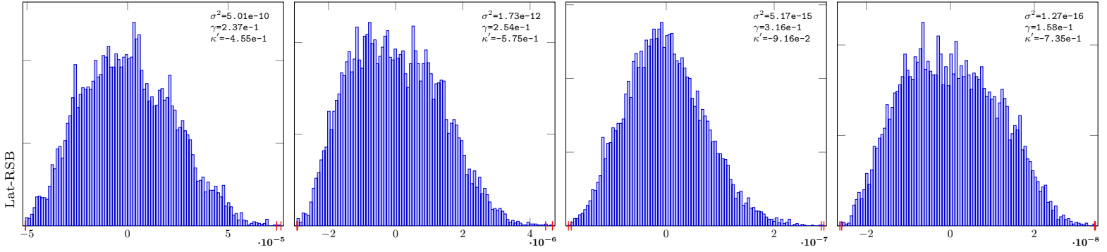
Gaussian-2-Lat-Rv-10
