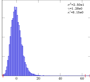
Gaussian-16-Sob-RDSB-12
