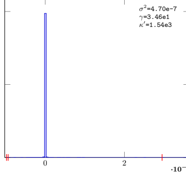
Gaussian-2-Lat-RpvRS-14
