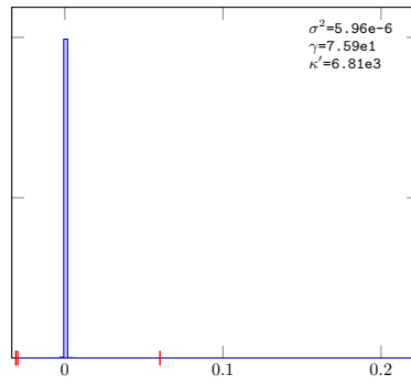
Gaussian-2-Lat-RpvRSB-14
