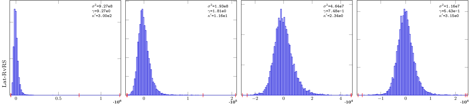
Gaussian-32-Lat-RvRSB-10
