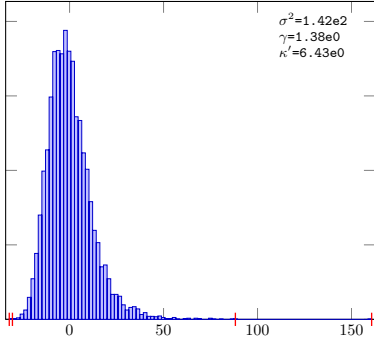
Gaussian-16-Sob-LMS-10
