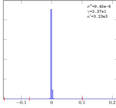
Gaussian-2-Lat-RvRSB-14
