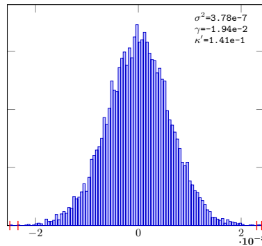
PieceLinGauss-16-Sob-LMS-RDS-14
