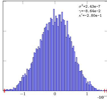
PieceLinGauss-8-Sob-LMS-14
