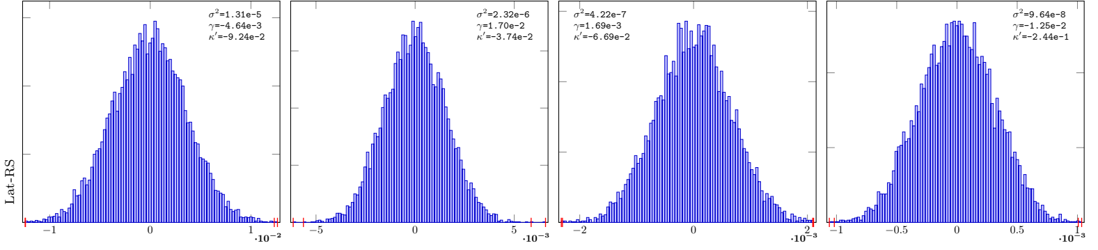
PieceLinGauss-8-Lat-RSB-10
