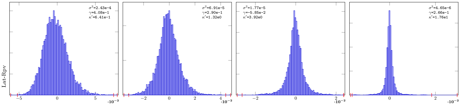
PieceLinGauss-16-Lat-Rpv-10
