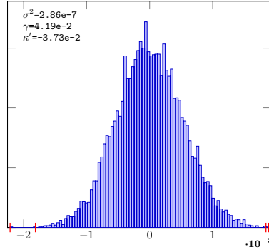
PieceLinGauss-16-Sob-RDSB-14
