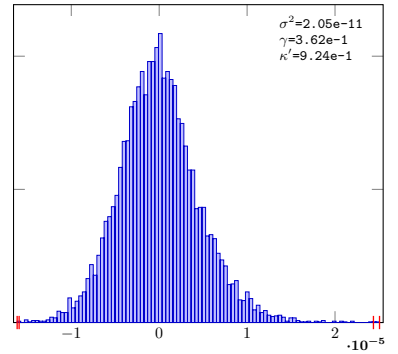
PieceLinGauss-2-Sob-LMS-RDS-16
