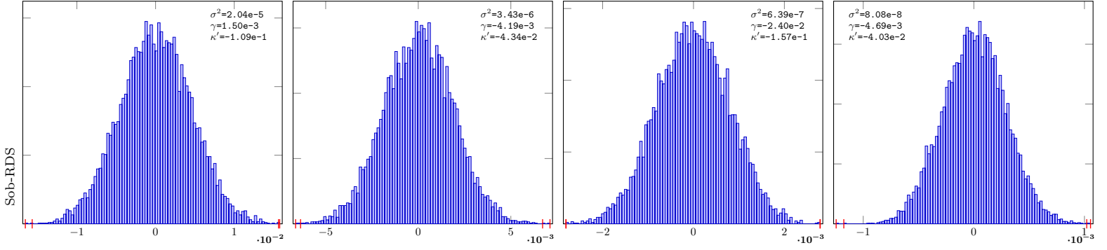
PieceLinGauss-32-Sob-RDSB-10
