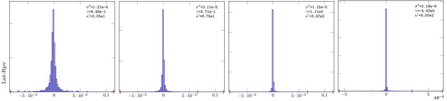
PieceLinGauss-2-Lat-Rpv-10
