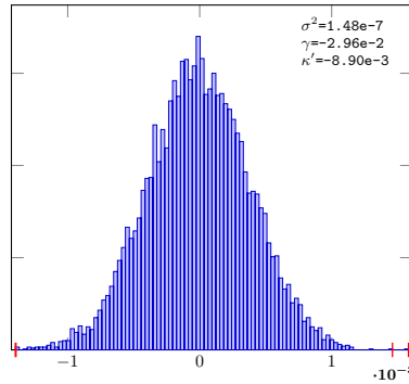
PieceLinGauss-8-Sob-LMS-RDS-14
