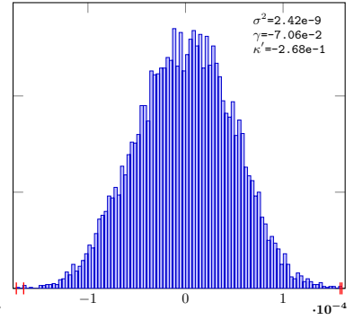
PieceLinGauss-4-Lat-Rv-16
