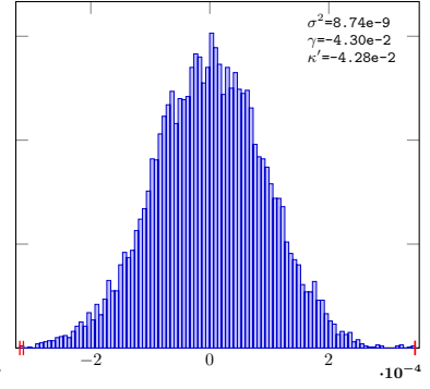
PieceLinGauss-4-Lat-RSB-16
