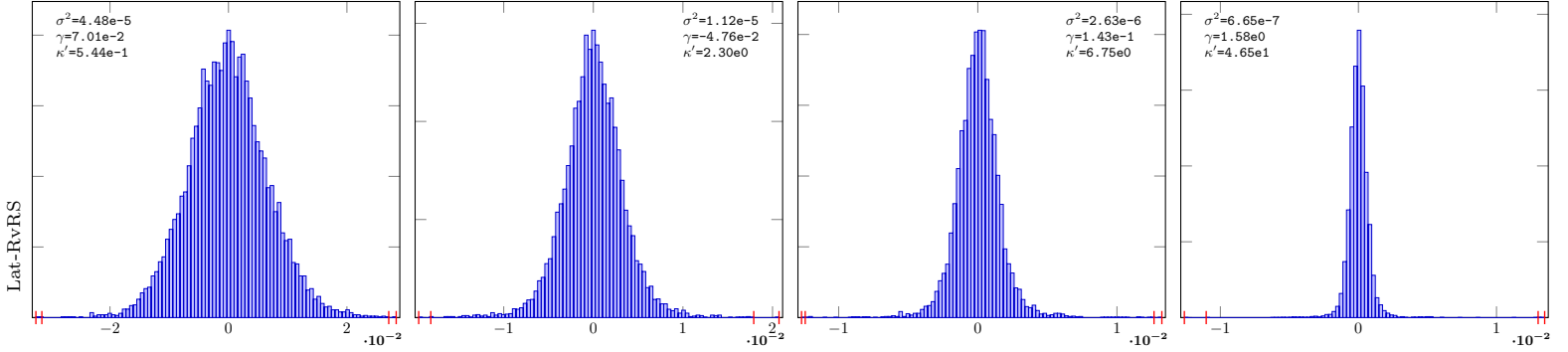
PieceLinGauss-16-Lat-RvRSB-10
