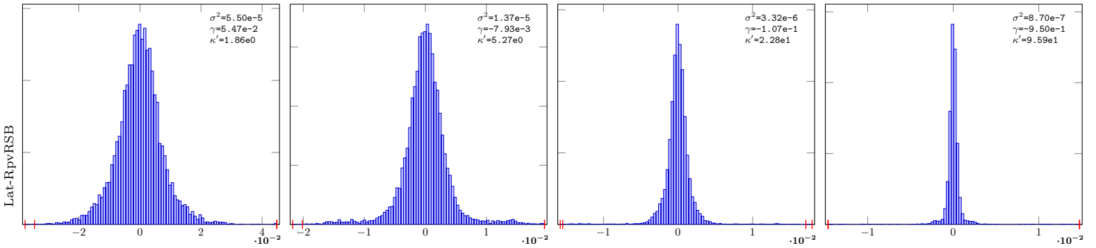
PieceLinGauss-16-Lat-RpvRSB-10
