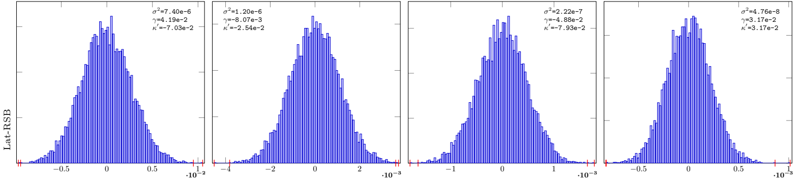
PieceLinGauss-32-Lat-Rv-10
