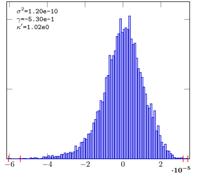
PieceLinGauss-2-Sob-LMS-16
