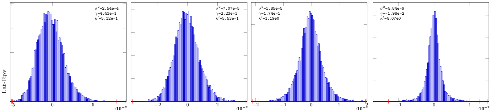
PieceLinGauss-32-Lat-Rpv-10
