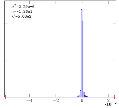
PieceLinGauss-4-Lat-Rpv-16
