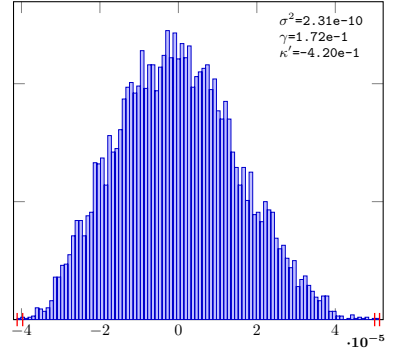
PieceLinGauss-2-Sob-RDSB-16
