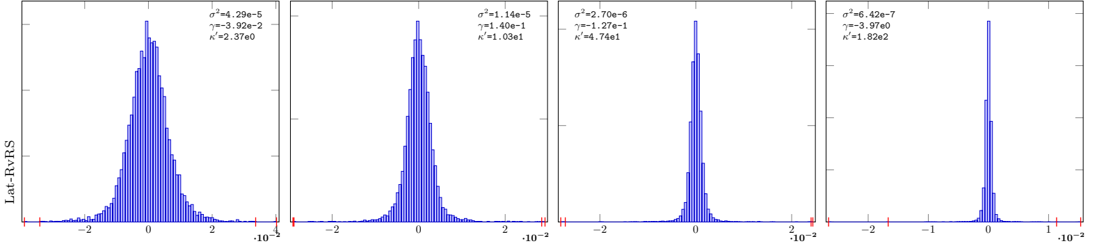
PieceLinGauss-8-Lat-RvRSB-10
