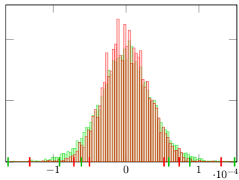
Sob-NUS, s = 16 , k = 14
