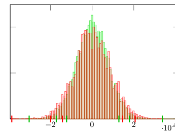
Sob-NUS, s = 16 , k = 16
