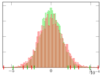
Sob-NUS, s = 16 , k = 12
