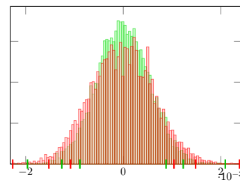
Sob-NUS, s = 16 , k = 10
