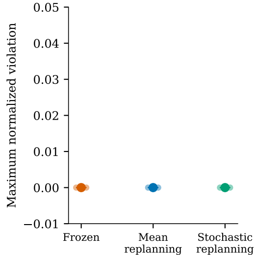
Constraint audit
