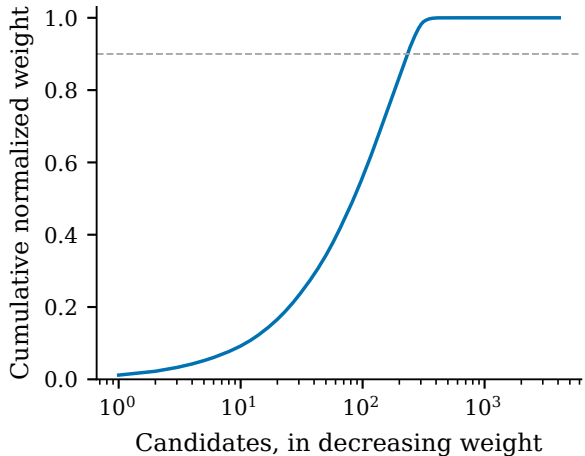
ESS = 225 of 4,096
