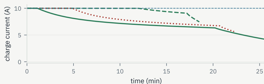
Governor action
