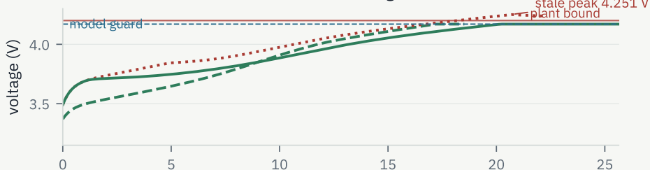
Terminal voltage
