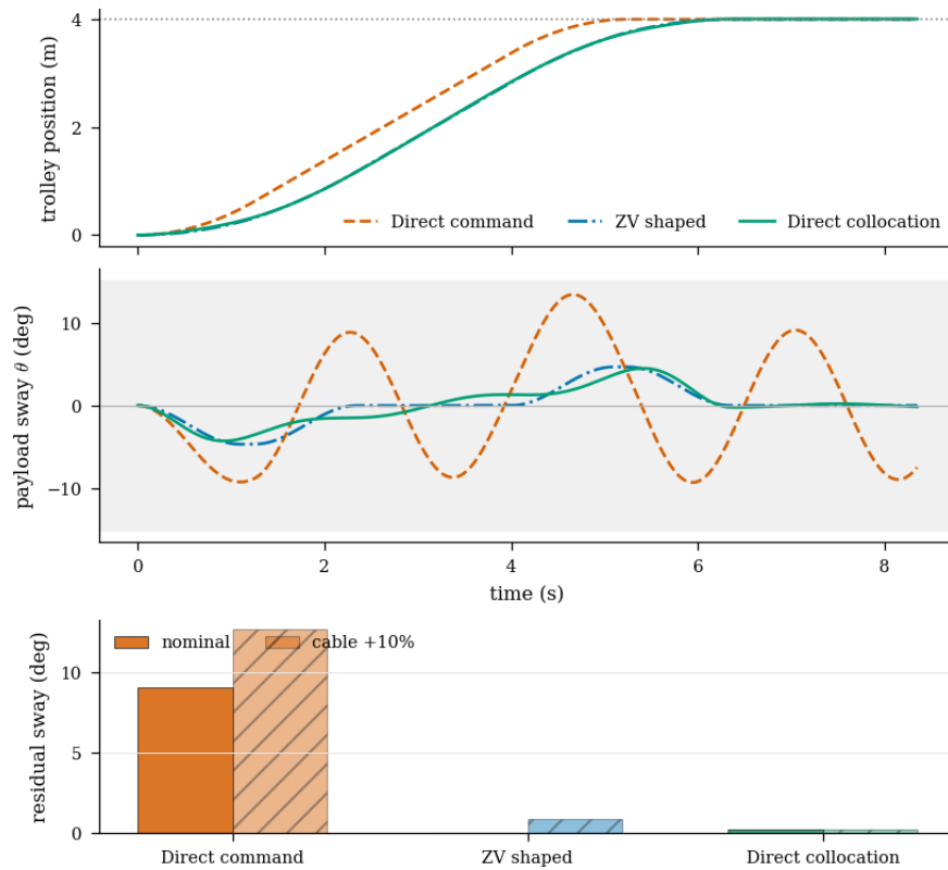
Figure 17: All three commands move the trolley through the same four-metre task on the nonlinear plant. The direct command leaves a large oscillation. The ZV shaper nearly cancels the nominal mode, while direct collocation reaches the terminal state with a smoother, lower-effort command. The lower panel replays the unchanged commands after increasing cable length by 10 percent. Hatched bars denote the mismatched plant.
