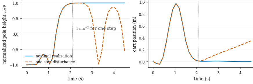
Figure 13: A one-step unmodeled acceleration separates two realizations driven by the same open-loop controls. The nominal trajectory reaches normalized pole height \cos \theta = 1 ; the disturbed trajectory finishes below the horizontal. The optimizer has produced a plan, not a rule that reacts to the observed state.
