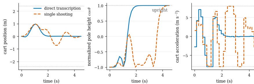
Figure 12: Direct transcription and single shooting solve the same nonlinear cart-pole problem from the same initialization. Both reach the upright configuration and respect the matched limits, but they converge to different local solutions. Direct transcription retains 154 scalar variables and 124 local dynamics equalities; single shooting retains only the 30 controls and reconstructs every state by forward simulation.
