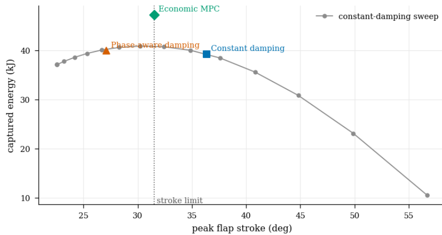
Figure 19: Captured energy against peak flap stroke. Gray circles sweep constant passive damping from 100 to 2800 N m s/rad. The vertical dotted line is the 0.55 rad stroke constraint. Economic MPC obtains more energy than the fixed-damping sweep by scheduling damping over the predicted wave cycle. The phase-aware baseline is feasible but does not attain the MPC energy.
