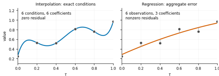
Figure 16: The panels use the same six values. On the left they are treated as six exact conditions for a degree-five interpolant, so every residual is zero. On the right they are treated as six observations for a three-parameter quadratic regression, so the fit trades errors across observations.
