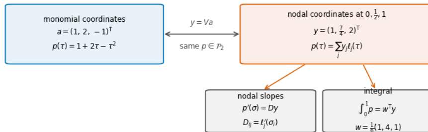
Figure 15: The same quadratic can be described by monomial coefficients or by its values at three support nodes. Direct collocation keeps the nodal coordinates. Fixed linear operators map those values to nodal derivatives and an integral; they are precomputed rather than optimized.
