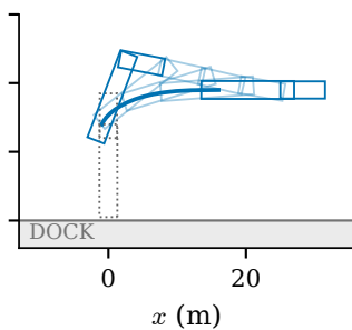
Iteration 3 Cost 2613.1
