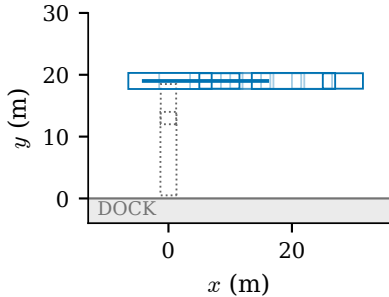
Iteration 0 Cost 5666.9
