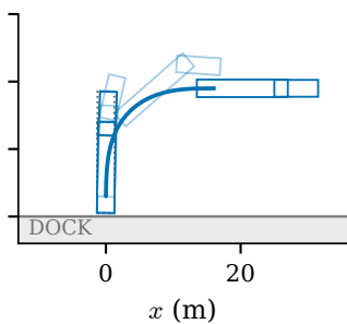
Iteration 821 Cost 12.2
