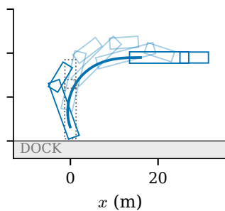
Iteration 10 Cost 69.2
