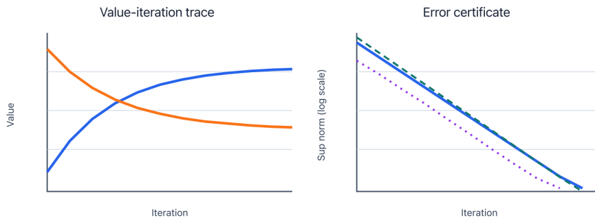
Figure 1: Static preview of value-iteration traces and a geometric contraction bound. The online book provides controls for \gamma , transitions, rewards, and the initial value.
