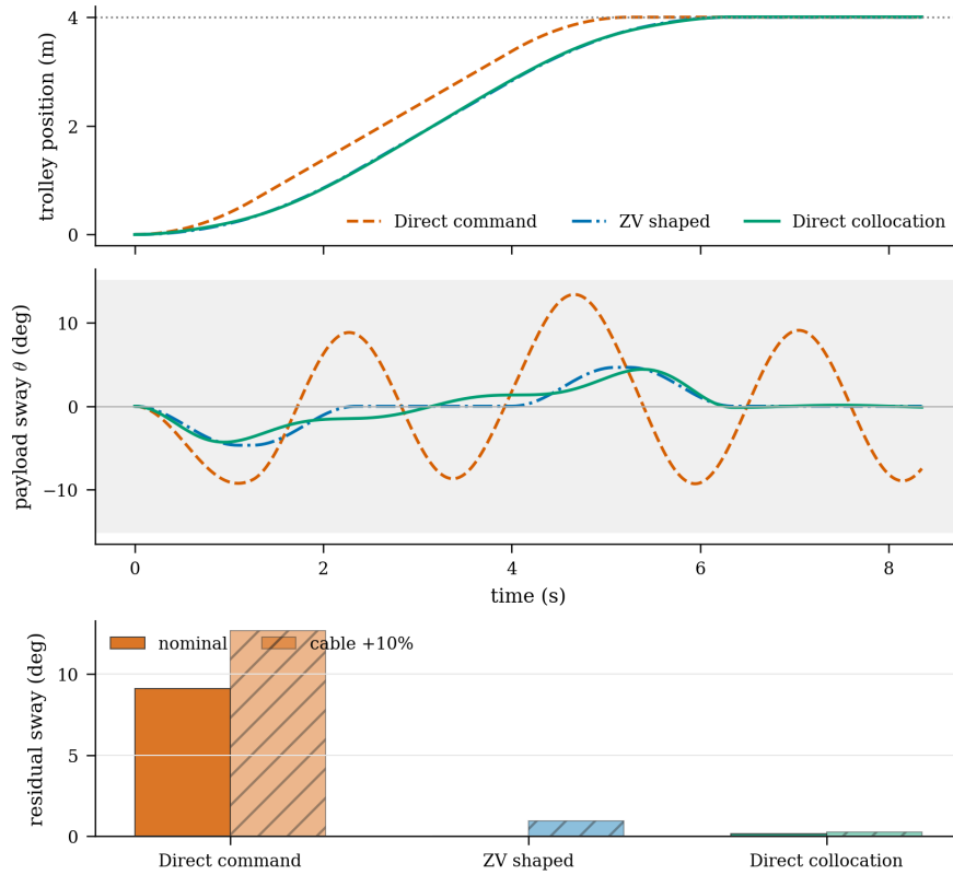
Figure 7: All three commands move the trolley through the same four-metre task on the nonlinear plant. The direct command leaves a large oscillation. The ZV shaper nearly cancels the nominal mode, while direct collocation reaches the terminal state with a smoother, lower-effort command. The lower panel replays the unchanged commands after increasing cable length by 10 percent. Hatched bars denote the mismatched plant.
