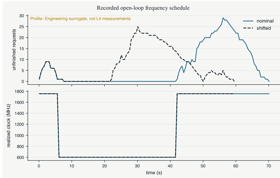
Figure 4: Static comparison of the nominal and shifted-burst replays. The online book adds playback and a controller selector.
