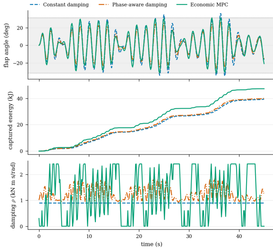
Figure 8: Closed-loop response under the same deterministic three-frequency forcing. The economic MPC captures more energy by varying passive damping and operating close to the stroke and PTO-torque limits. Constant damping crosses the shaded stroke-feasible region, while the phase-aware baseline stays farther inside it. Every curve is generated by the nonlinear plant simulation.
