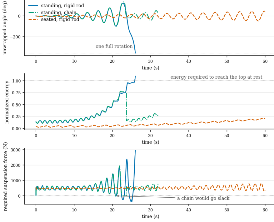
Figure 2: The structured standing controller completes a rotation on the rigid-rod plant, but that trajectory eventually requires a negative suspension force. SwingRL’s unilateral chain model clips the feasible force at zero, enters a ballistic phase, and does not complete a rotation under the same controller. The seated rigid-rod trajectory remains taut but does not rotate within 60 seconds.
