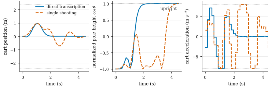
Figure 5: Direct transcription and single shooting solve the same nonlinear cart-pole problem from the same initialization. Both reach the upright configuration and respect the matched limits, but they converge to different local solutions. Direct transcription retains 154 scalar variables and 124 local dynamics equalities; single shooting retains only the 30 controls and reconstructs every state by forward simulation.
