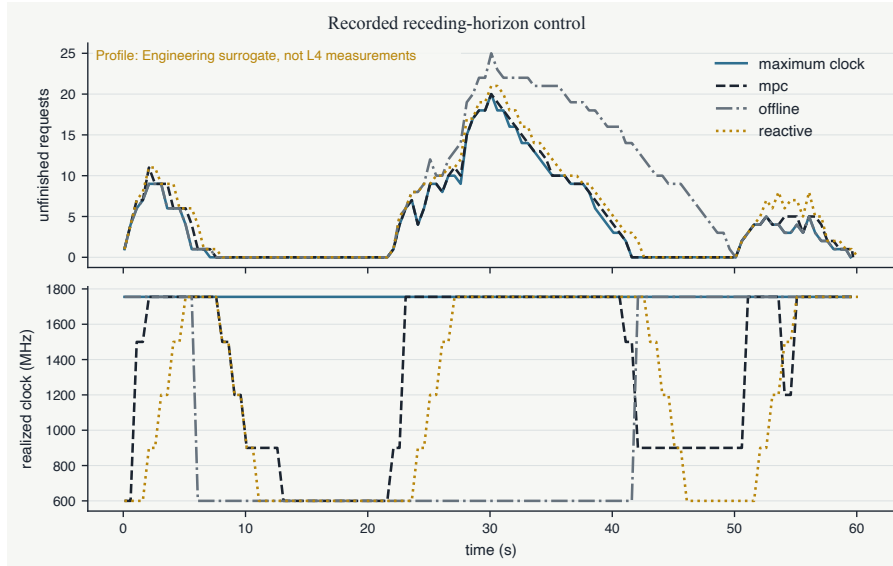
Figure 10: Static view of the closed-loop comparison. The online book provides playback and exposes the planned MPC horizon available at each control time.
