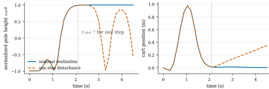
Figure 6: A one-step unmodeled acceleration separates two realizations driven by the same open-loop controls. The nominal trajectory reaches normalized pole height \cos \theta = 1 ; the disturbed trajectory finishes below the horizontal. The optimizer has produced a plan, not a rule that reacts to the observed state.
