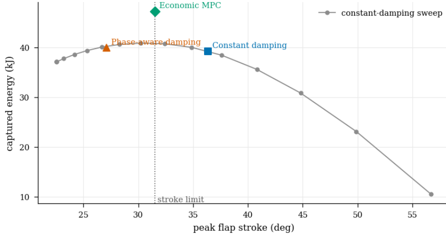
Figure 13: Captured energy against peak flap stroke. Gray circles sweep constant passive damping from 100 to 2800 N m s/rad. The vertical dotted line is the 0.55 rad stroke constraint. Economic MPC obtains more energy than the fixed-damping sweep by scheduling damping over the predicted wave cycle. The phase-aware baseline is feasible but does not attain the MPC energy.
