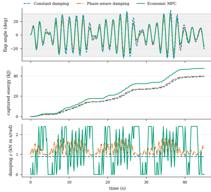
Figure 12: Closed-loop response under the same deterministic three-frequency forcing. The economic MPC captures more energy by varying passive damping and operating close to the stroke and PTO-torque limits. Constant damping crosses the shaded stroke-feasible region, while the phase-aware baseline stays farther inside it. Every curve is generated by the nonlinear plant simulation.
