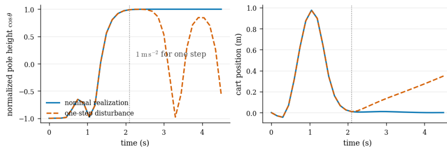
Figure 10: A one-step unmodeled acceleration separates two realizations driven by the same open-loop controls. The nominal trajectory reaches normalized pole height \cos \theta = 1 ; the disturbed trajectory finishes below the horizontal. The optimizer has produced a plan, not a rule that reacts to the observed state.
