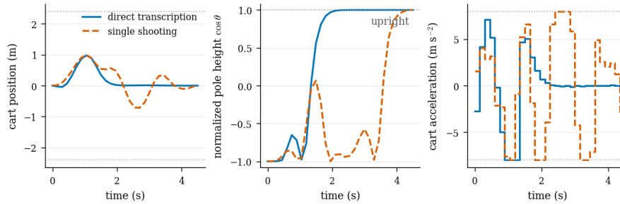
Figure 9: Direct transcription and single shooting solve the same nonlinear cart-pole problem from the same initialization. Both reach the upright configuration and respect the matched limits, but they converge to different local solutions. Direct transcription retains 154 scalar variables and 124 local dynamics equalities; single shooting retains only the 30 controls and reconstructs every state by forward simulation.
