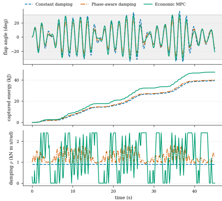
Figure 13: Closed-loop response under the same deterministic three-frequency forcing. The economic MPC captures more energy by varying passive damping and operating close to the stroke and PTO-torque limits. Constant damping crosses the shaded stroke-feasible region, while the phase-aware baseline stays farther inside it. Every curve is generated by the nonlinear plant simulation.
