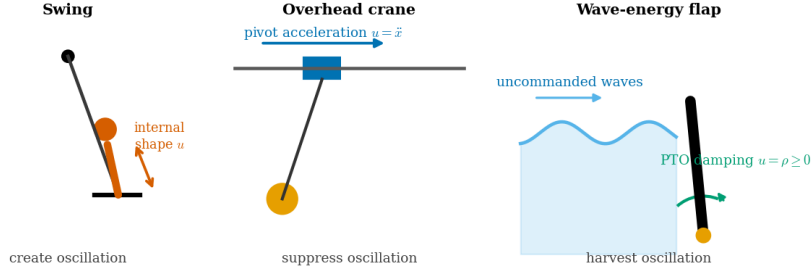
Figure 1: The systems share an oscillatory silhouette but expose different control interfaces. The rider changes internal shape, the crane accelerates its pivot, and the wave device changes a nonnegative dissipative load. Their desired motions and feasible actions therefore differ.
