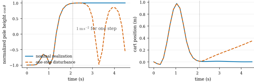
Figure 11: A one-step unmodeled acceleration separates two realizations driven by the same open-loop controls. The nominal trajectory reaches normalized pole height \cos \theta = 1 ; the disturbed trajectory finishes below the horizontal. The optimizer has produced a plan, not a rule that reacts to the observed state.
