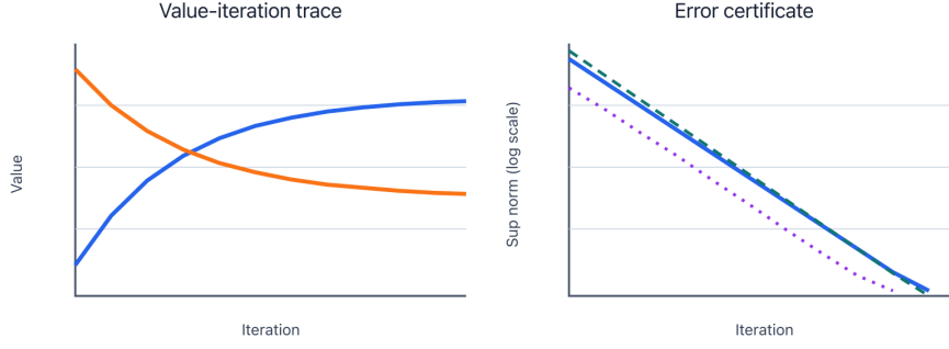
Figure 17: Static preview of value-iteration traces and a geometric contraction bound. The online book provides controls for \gamma , transitions, rewards, and the initial value.
