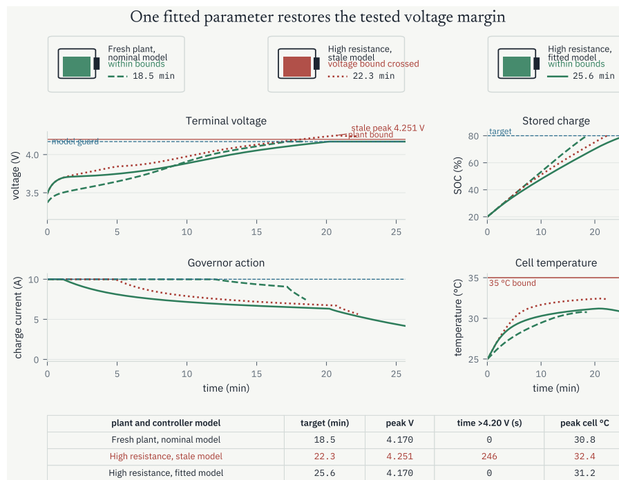
Figure 8: The stale model loses its voltage margin after resistance changes. Updating one fitted resistance scale restores the tested margin at the cost of a longer charge. The online book adds synchronized playback and event seeking.
