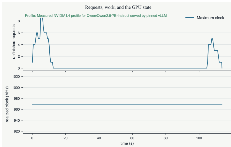
Figure 6: Static summary of unfinished requests and realized clock from the same request-level simulation. The online book provides playback, stepping, scrubbing, phase detail, and controller selection.
