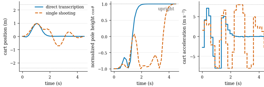
Figure 10: Direct transcription and single shooting solve the same nonlinear cart-pole problem from the same initialization. Both reach the upright configuration and respect the matched limits, but they converge to different local solutions. Direct transcription retains 154 scalar variables and 124 local dynamics equalities; single shooting retains only the 30 controls and reconstructs every state by forward simulation.
