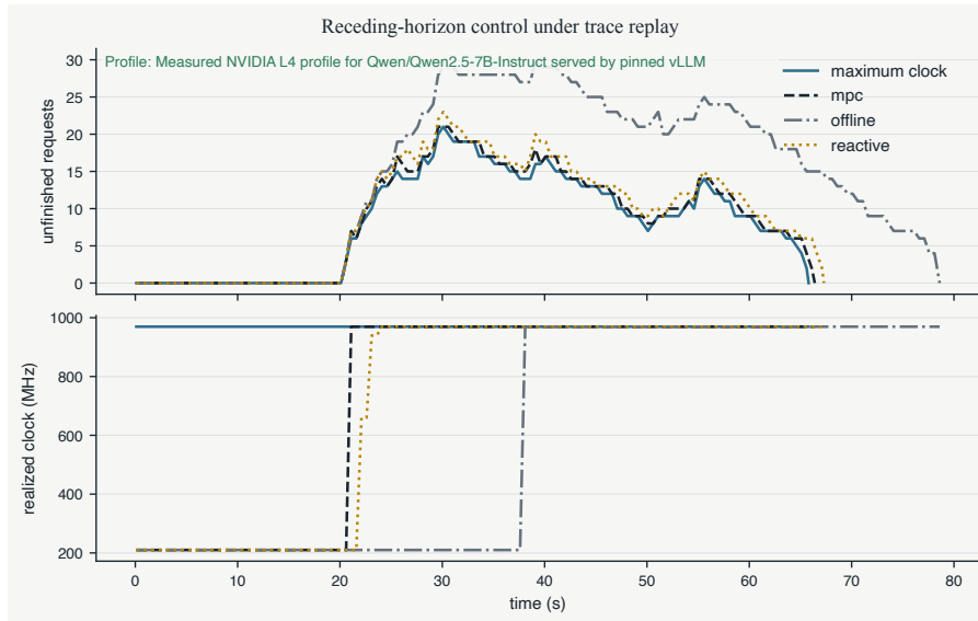
Figure 15: Static view of the closed-loop comparison. The online book provides playback and exposes the planned MPC horizon available at each control time.
