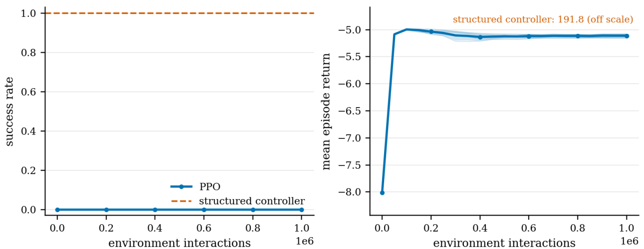
Figure 20: Five prespecified PPO seeds evaluated on the same 100 fixed initial states. Thin blue traces show individual seeds; the solid trace and band show the mean and a two-sided 95% t interval with seed as the statistical unit. PPO improves its return early but never completes a rotation. The structured controller succeeds from every state and obtains mean return 191.8; this value is annotated off scale in the return panel so that the smaller PPO change remains visible.
