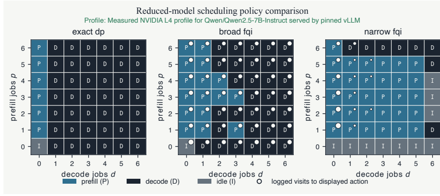
Figure 19: Static policy slices for oldest-age bin four. At each displayed state, a white circle marks that the buffer contains visits to the action selected by the displayed policy. The interactive version adds age selection, playback, stepping, and scrubbing through a queue trajectory sampled from the reduced transition model rather than observed directly from vLLM.
