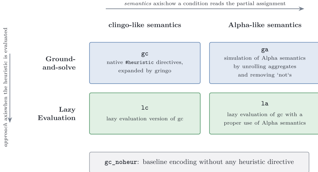
Figure 2: The experimental matrix. Prefixes name the approach, suffixes the semantics.
