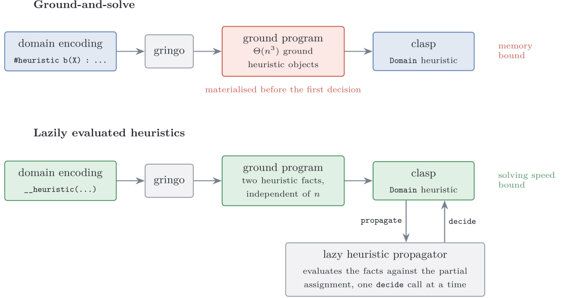
Figure 1: The same heuristic under the two approaches compared in this thesis.
