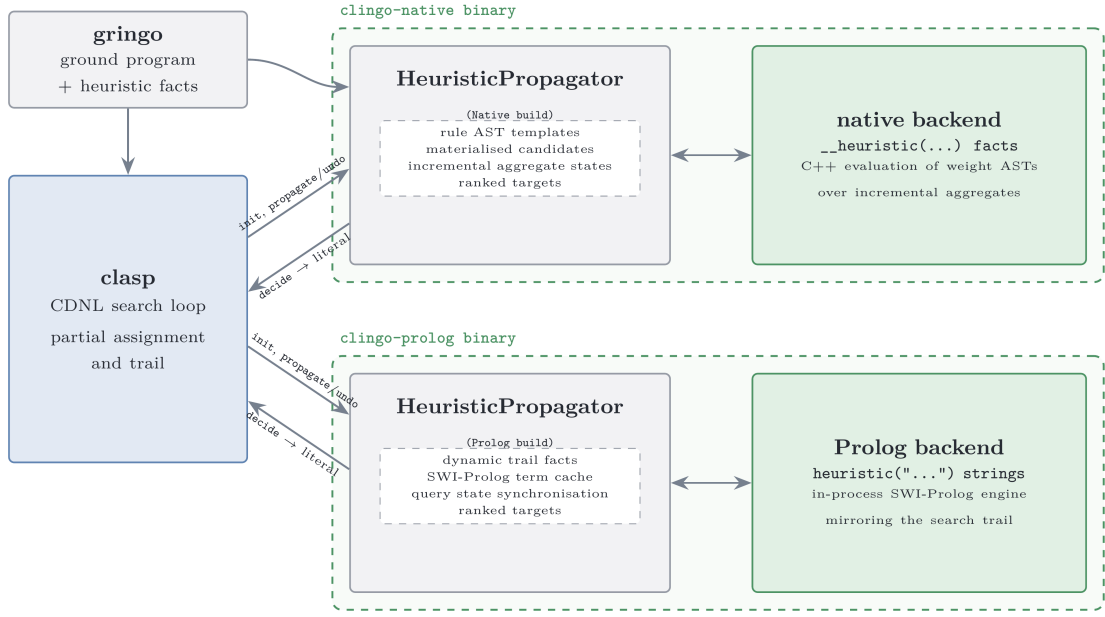
Figure 3: System architecture of the two binary variants ( clingo-native and clingo-prolog ), showing their respective heuristic propagators and evaluation backends attached to clasp .
