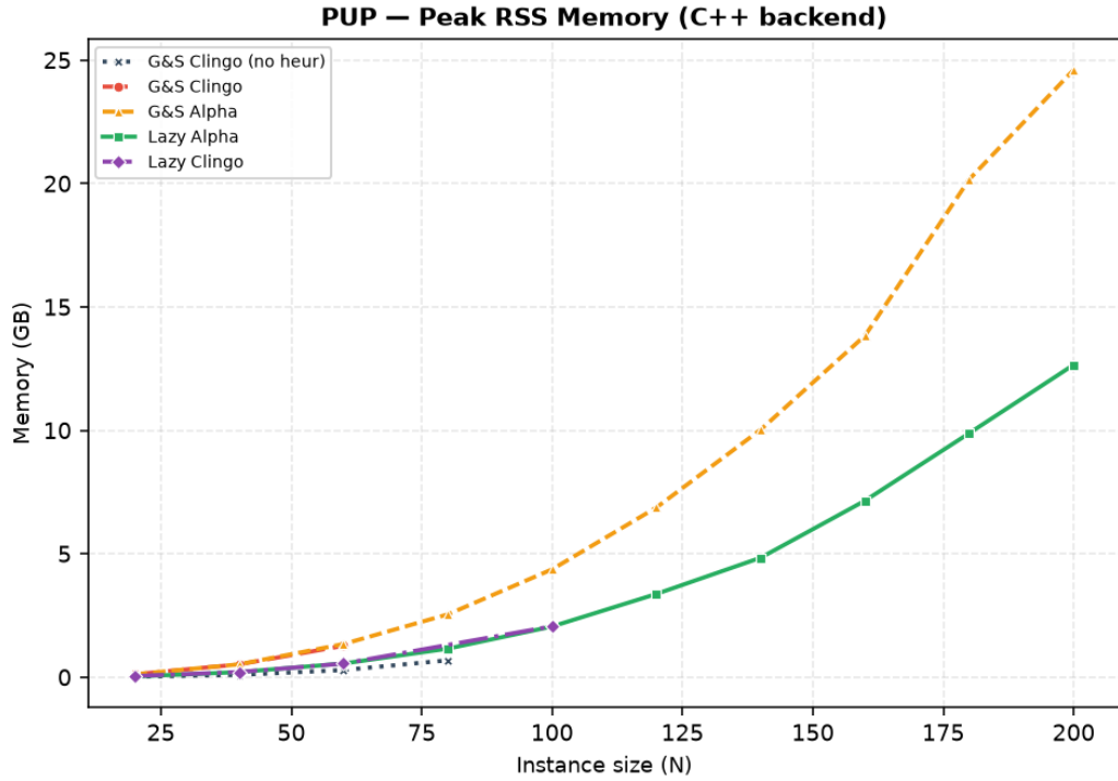
Figure 4.13: Peak memory usage on PUP for the C++ backend, illustrating the 2\times memory reduction of la over ga .
