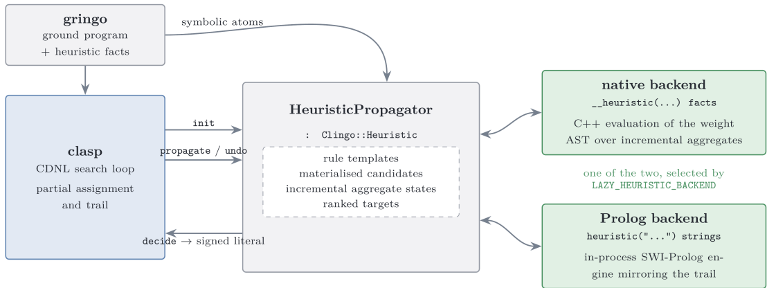
Figure 3: The heuristic propagator between clasp and the two evaluation backends.
