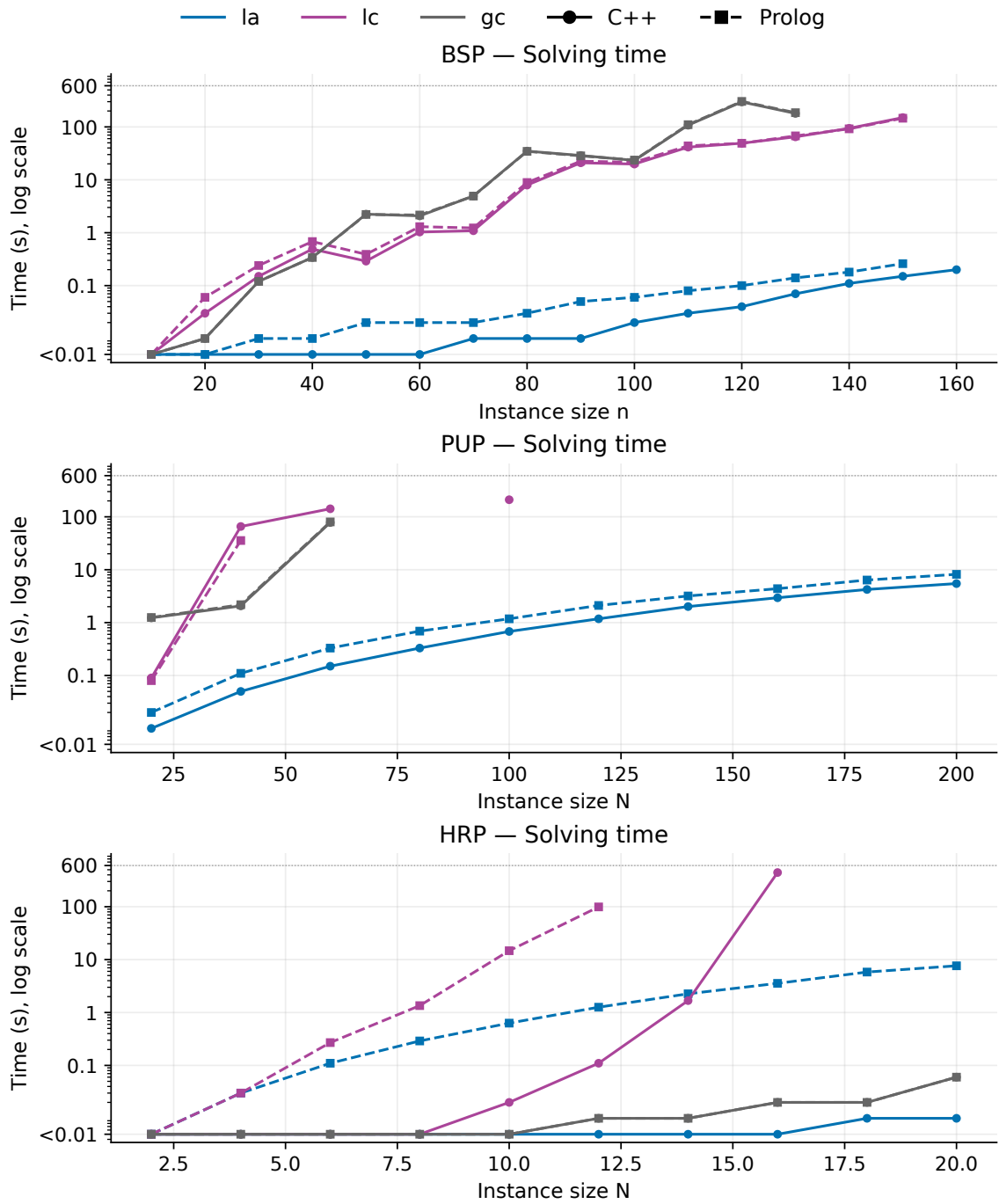
Figure 4.13: Solving time on both backends for 1a, 1c and the ground control gc. Colour identifies the variant; solid circles denote C++ and dashed squares Prolog. Only successful runs are plotted. The dotted line marks 600s for orientation, although the actual budget includes grounding as well. Values reported below 0.01 s are shown at a plotting floor.
