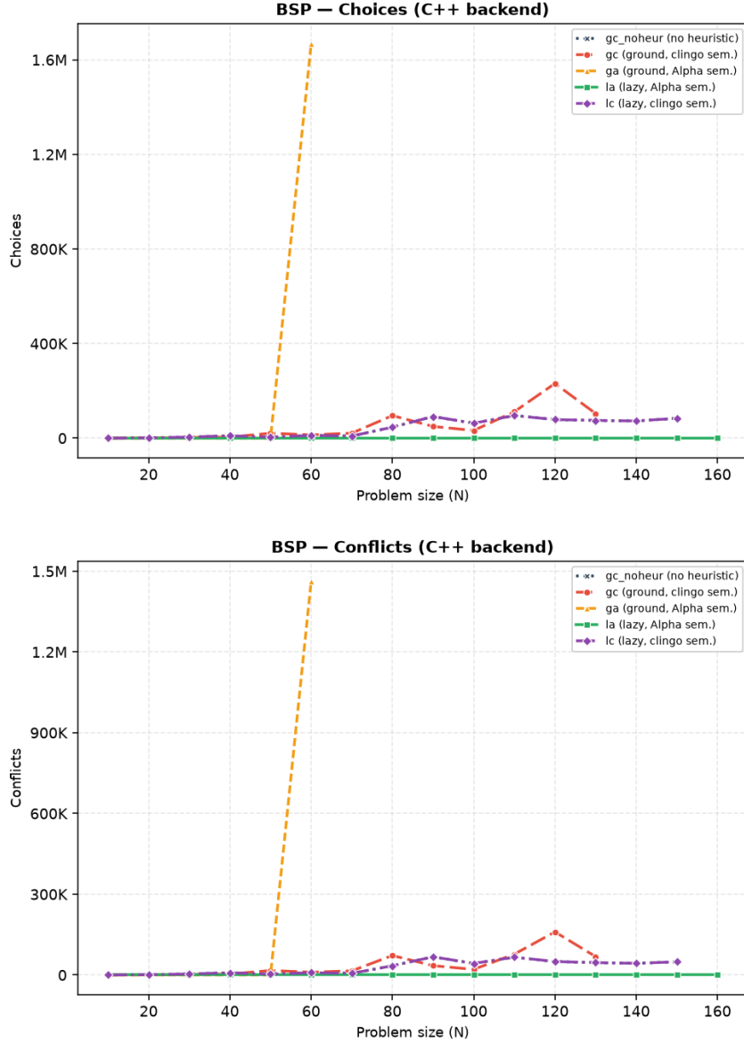
Figure 4.5: BSP search statistics on the C++ backend: solver choices (top) and conflicts (bottom) across sizes.
