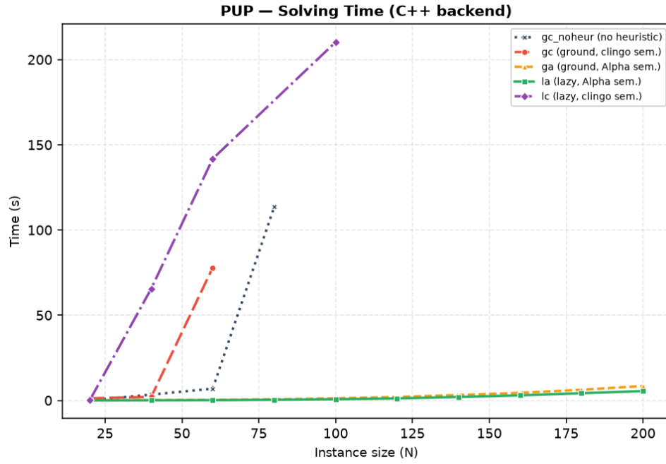
Figure 4.8: Solving time on PUP for the C++ backend.
