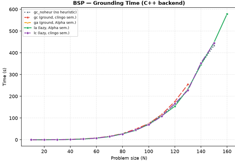
Figure 4.2: Grounding time on BSP for the C++ backend. One run per point; a curve ends where its variant stops solving within the limits.
