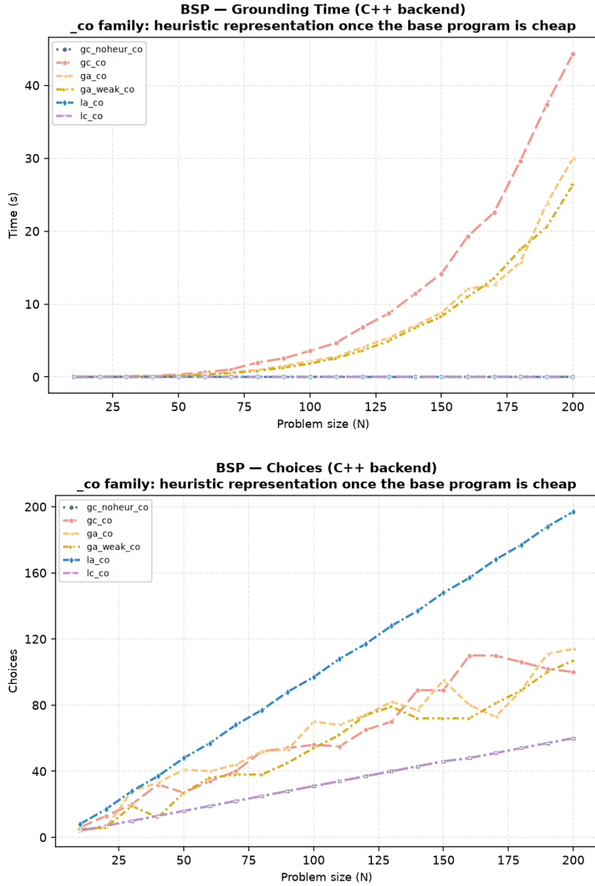
Figure 4.23: The _co family on BSP: grounding time (top) and solver choices (bottom). The ground and the lazy variants separate on grounding by three orders of magnitude.
