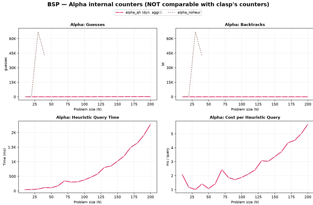
Figure 4.17: BSP internal search counters for Alpha across instance sizes. Top row: with heuristics ( alpha_qh ), guesses remain equal to n with zero backtracks; without heuristics ( alpha_noheur ), search explodes past n = 20 and the curve stops at n = 40 , the last size it solves. Bottom row: cumulative Prolog query evaluation time for alpha_qh , which reaches 2.3 s at n = 200 and never costs more than 5.7 ms per consultation.
