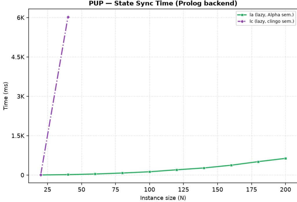
Figure 4.15: Cumulative state synchronization time for the Prolog backend on PUP, with true_atom/1 and false_atom/1 as foreign predicates. For 1a it grows smoothly to 0.63s at N = 200 , below the 3.25s the same run spends inside the Prolog query; the 1c curve, which pays one update per literal on an unguided search, reaches 6s already at N = 40 and stops there.
