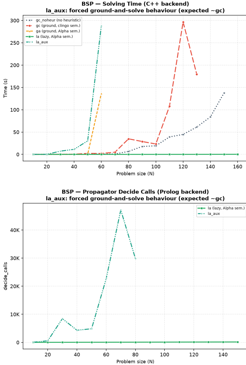
Figure 4.21: Solving time on the C++ backend (top) and number of propagator decide calls on the Prolog backend (bottom) comparing la_aux against direct la in BSP.
