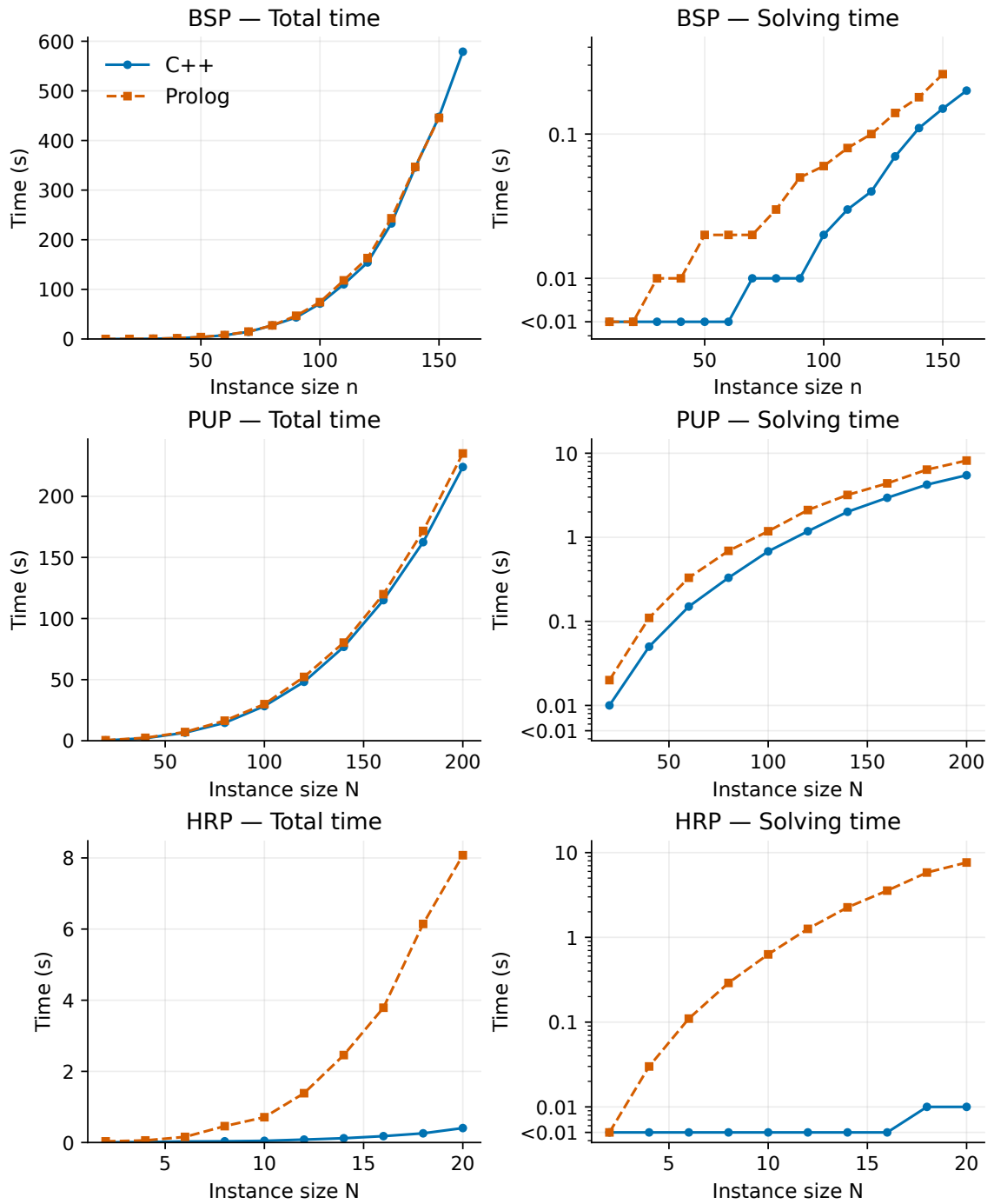
Figure 4.12: The 1a variant on C++ and Prolog across all three families: total clingo time (left) and solving time (right). Each panel has its own vertical scale; the solving panels use a logarithmic scale to keep both backends visible. Only successful runs are plotted, and curves end at the largest solved instance.
