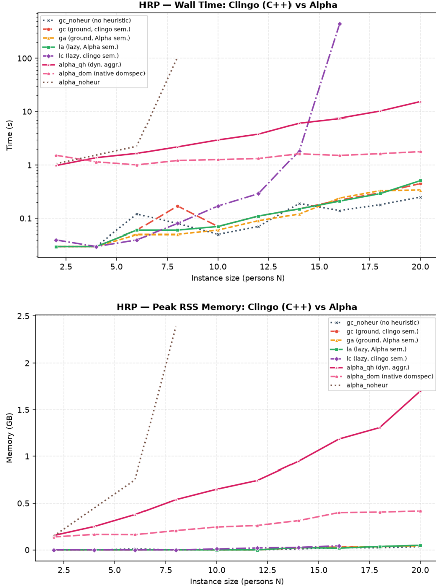
Figure 4.19: HRP benchmark dashboard: the clingo variants against Alpha in all three configurations, including alpha_dom . Top: total wall-clock time, on a logarithmic scale to keep the sub-second clingo runs visible next to alpha_noheur ; bottom: peak RSS. Both are runlim external process measures, and Alpha’s RSS includes the resident JVM. Only successful runs are plotted, so lc ends at N = 16 and alpha_noheur at N = 8 .
