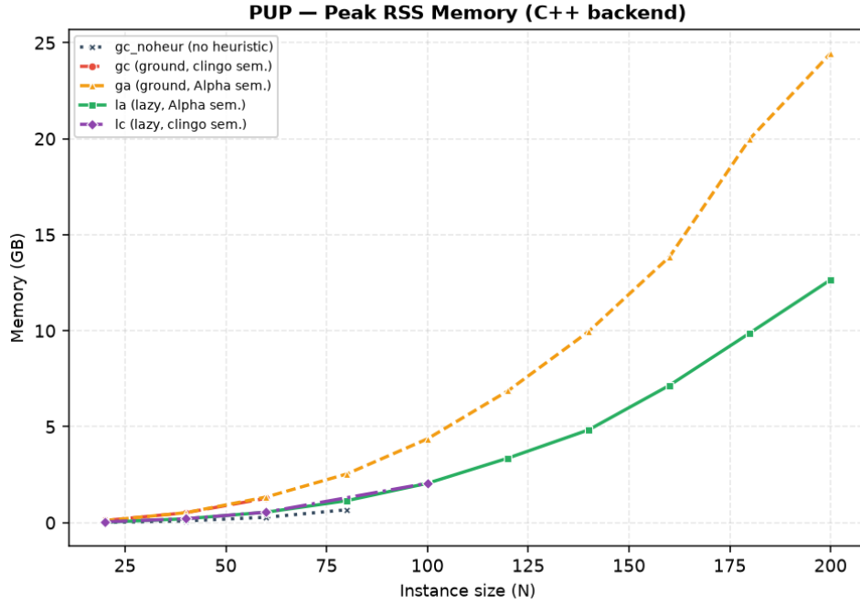
Figure 4.10: Peak memory usage on PUP for the C++ backend, illustrating the 2\times memory reduction of la over ga .
