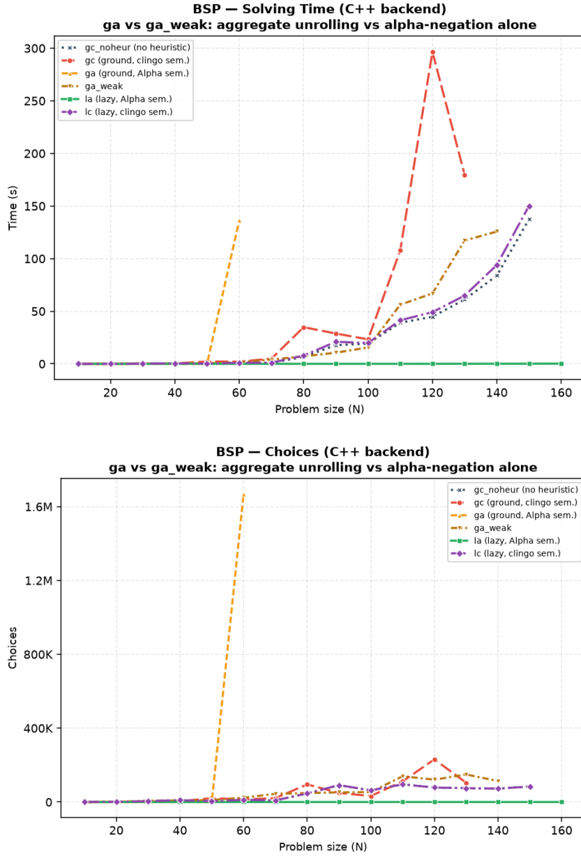
Figure 4.20: Solving time (top) and solver choices (bottom) for BSP comparing the Alpha-like semantics simulations ( ga and ga_weak ) against the baseline variants.
