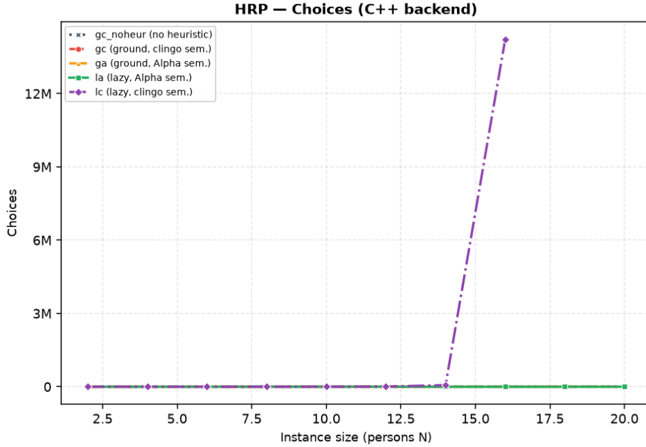
Figure 4.11: HRP: solver choices on the C++ backend. The only diverging curve is lc , analyzed in Section 4.10.
