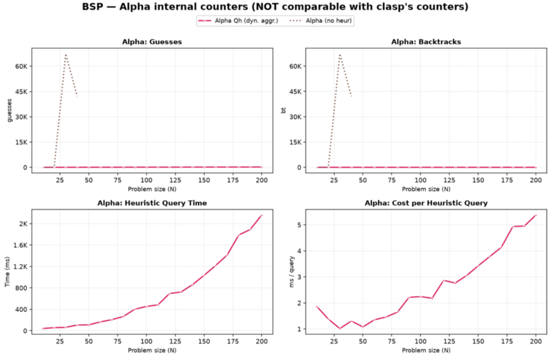
Figure 4.18: BSP, Alpha’s own counters, plotted apart from every clingo measure because they are not commensurable with clasp’s (Section 3.3.4). Top row: with the heuristic, guesses stay equal to n and backtracks at zero over the whole range, while the heuristic-free run spikes to some 67,000 of each at n = 30 and stops at n = 40 . Bottom row: the cost of the heuristic itself, which is a Prolog query in this variant — 2.2 seconds cumulative at n = 200 , at 1.9 to 5.4 milliseconds per query.
