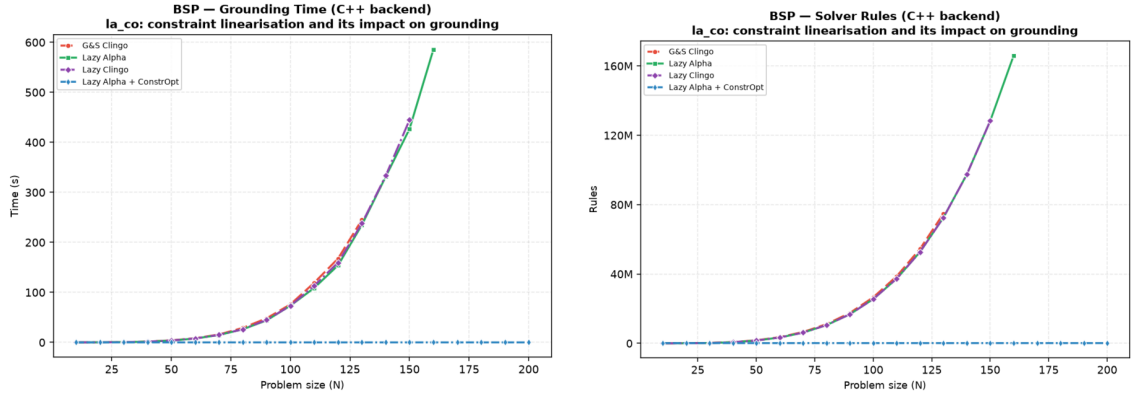
Figure 4.10: BSP, C++ backend, exploratory comparison of the constraint reformulation: grounding time (left) and propositional rules (right). gc , 1a , and 1c overlap because they share the quadratic base encoding (some 52.8 million rules and one to three minutes of grounding at n = 120 ); 1a_co lies on the horizontal axis of both plots (366 rules, milliseconds of grounding), the visual form of the five-orders-of-magnitude gap discussed in the text.
