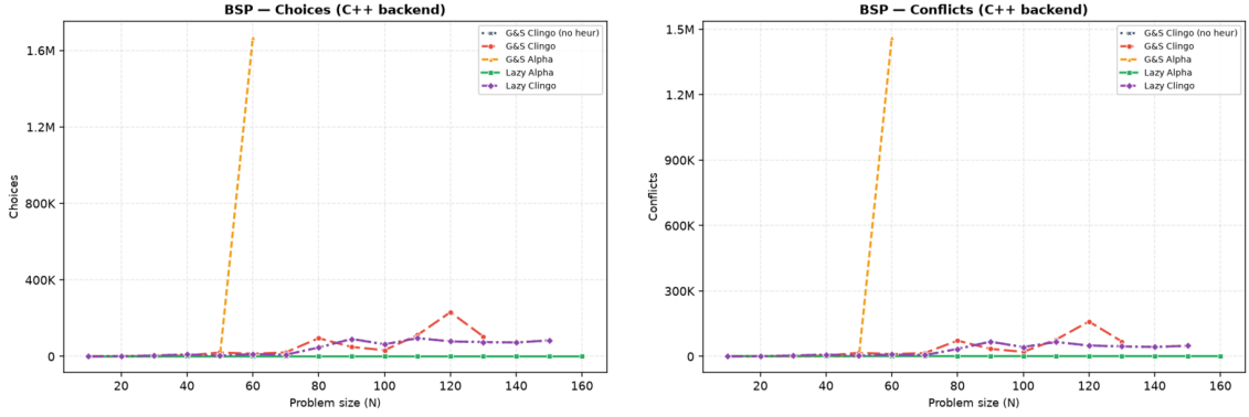
Figure 4.4: BSP, C++ backend: choices and conflicts. 1a lies on the horizontal axis; 1c coincides with the baseline exactly, at every size both solve, so the two curves are superimposed; ga leaves the chart after n = 60 . Unlike the time plots, these are exact structural counts.
