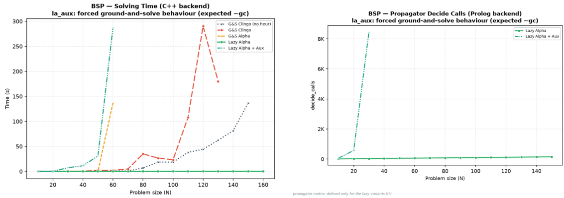
Figure 4.9: BSP, exploratory comparison of the auxiliary form. Left: C++ solving time; 1a_aux diverges from n = 40 and leaves the chart after n = 60 , while the direct 1a stays on the axis. Right: propagator decide calls on the Prolog backend; the auxiliary candidates multiply the consultations (573 at n = 20 and 8,452 at n = 30 , against the n calls of the direct form), and the curve ends at n = 30 , the last size the variant solves on that backend.
