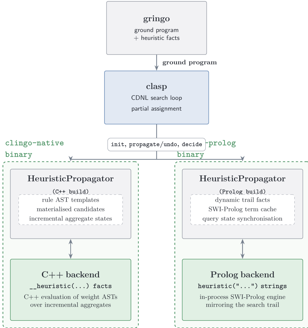
Figure 3: System architecture of the two binary variants ( clingo-native and clingo-prolog ), showing their respective heuristic propagators and evaluation backends attached to clasp.
