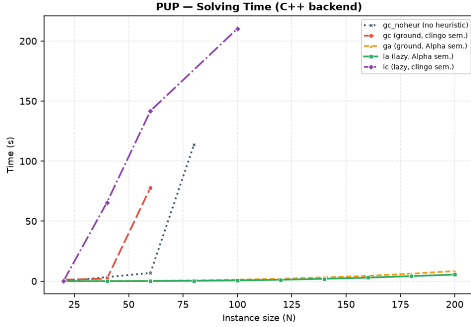
Figure 5.8: Solving time on PUP for the C++ backend.
