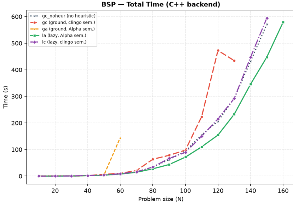
Figure 5.4: BSP total time, grounding plus solving, on the C++ backend.
