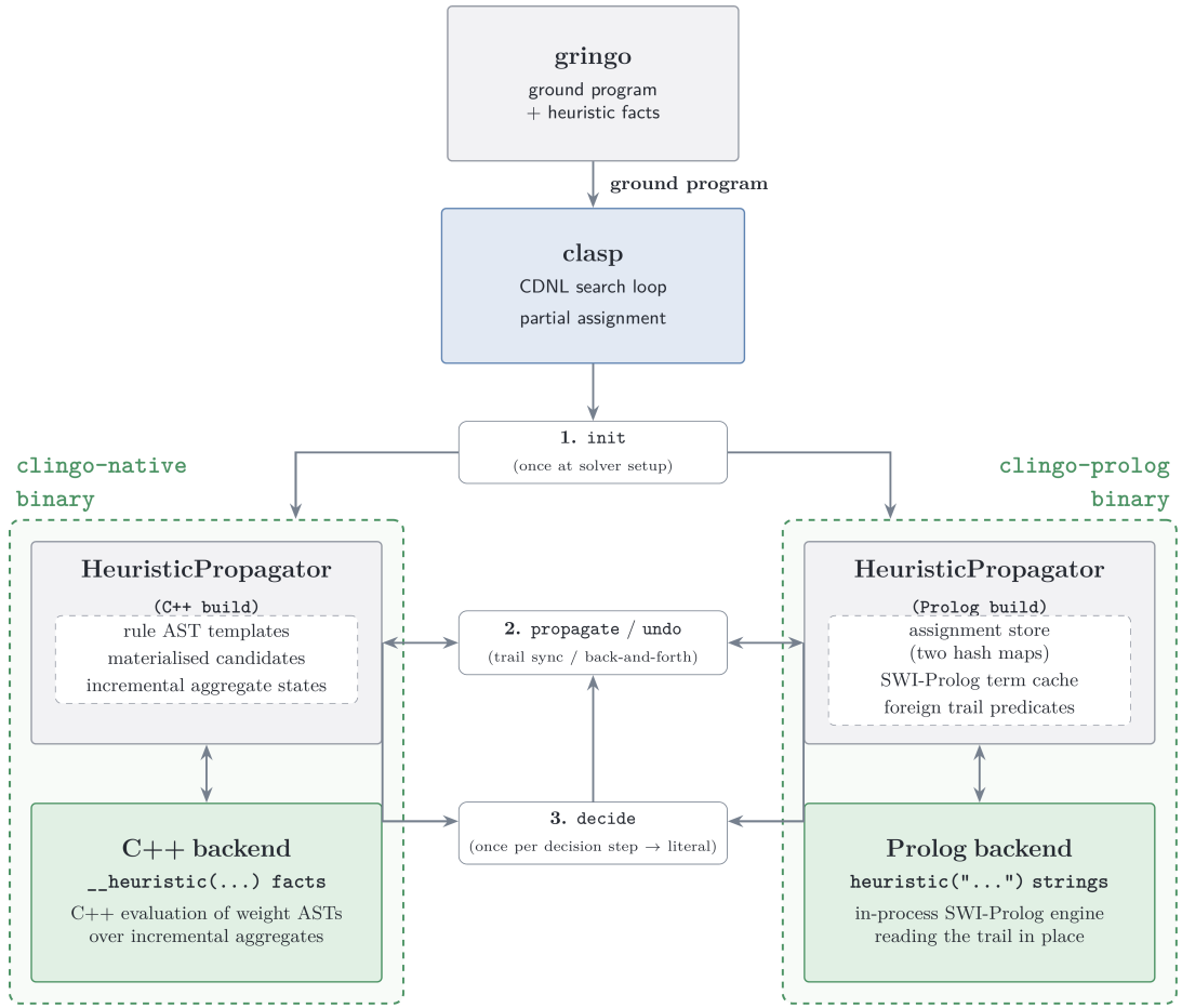
Figure 3.2: System architecture of the two binary variants, showing their respective heuristic propagators and evaluation backends attached to clasp.
