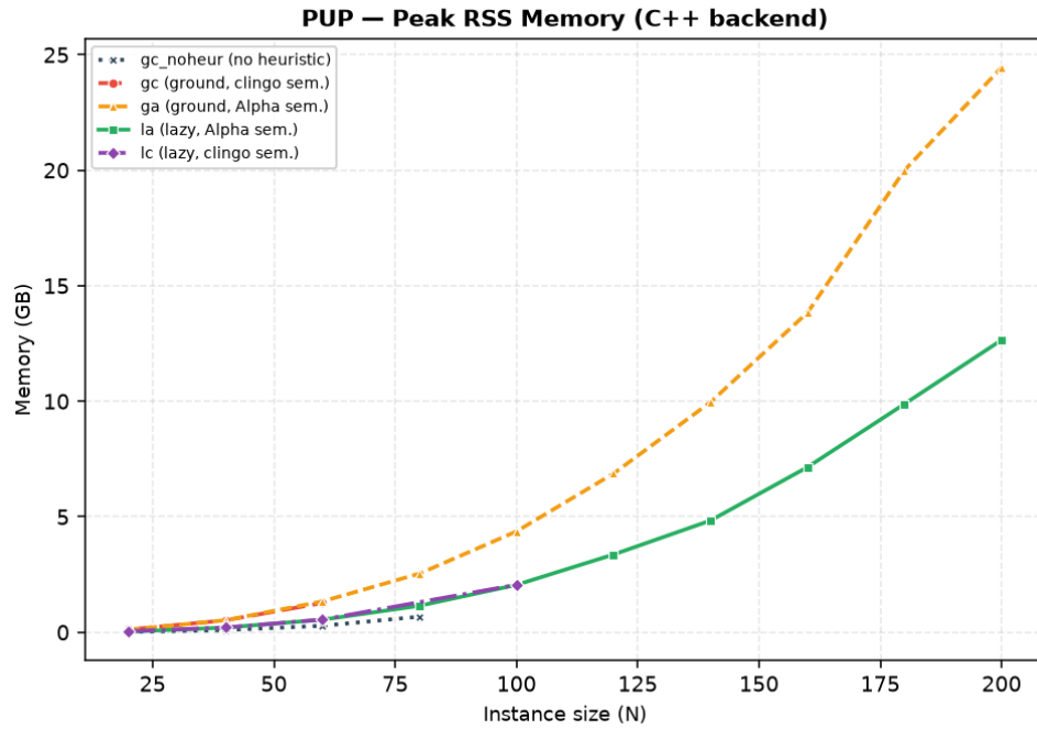
Figure 5.10: Peak memory usage on PUP for the C++ backend, illustrating the 2× memory reduction of la over ga.
