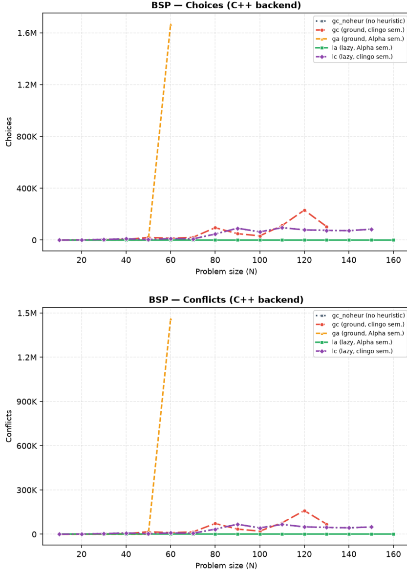
Figure 5.5: BSP search statistics on the C++ backend: solver choices (top) and conflicts (bottom) across sizes.
