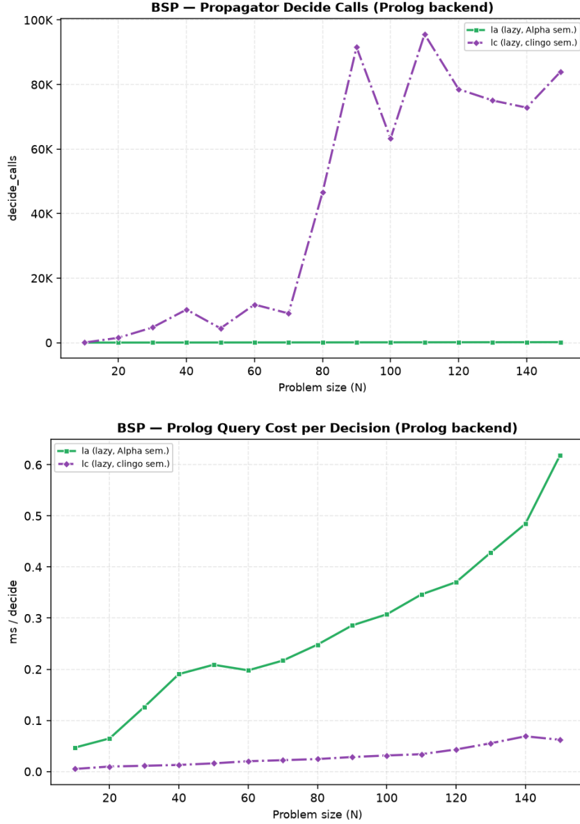
Figure 5.14: BSP, Prolog backend: decide calls (top) and per-decision query cost (bottom). The 1c curve pairs tens of thousands of calls with a low unit cost; 1a the opposite.
