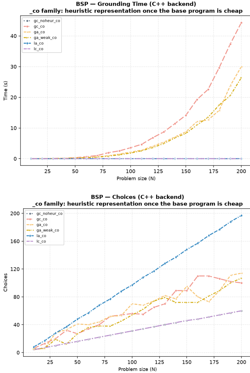
Figure 5.23: The _co family on BSP: grounding time (top) and solver choices (bottom). The ground and the lazy variants separate on grounding by three orders of magnitude.
