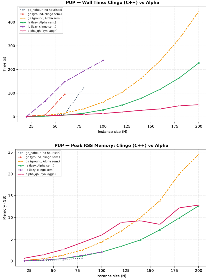
Figure 5.18: PUP benchmark dashboard: external comparison between clingo variants and Alpha. Top: total wall-clock time; bottom: peak RSS. The baseline alpha_noheur does not appear as it solves zero instances; the lc line connects successful runs across the timeout at N = 80 .
