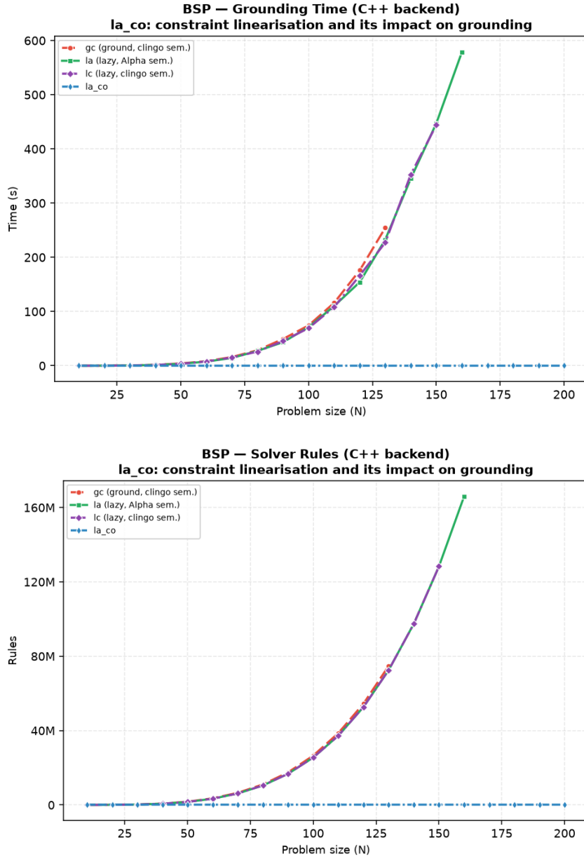
Figure 5.22: Grounding time (top) and propositional rule count (bottom) for BSP on the C++ backend, comparing the compact constraint formulation ( la co ) against the baseline encodings ( gc , la , and lc ).
