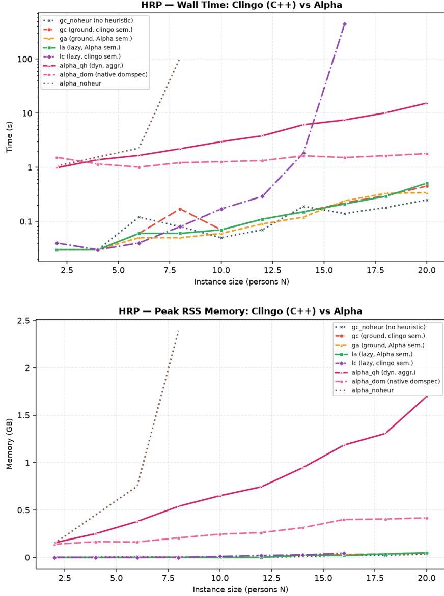
Figure 5.19: HRP benchmark dashboard: the clingo variants against Alpha in all three configurations, including alpha_dom . Top: total wall-clock time, on a logarithmic scale to keep the sub-second clingo runs visible next to alpha_noheur ; bottom: peak RSS. Both are runlim external process measures, and Alpha’s RSS includes the resident JVM. Only successful runs are plotted, so lc ends at N = 16 and alpha_noheur at N = 8 .
