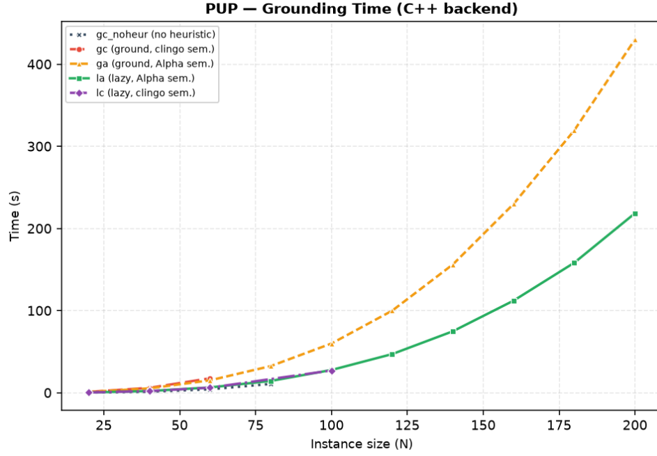
Figure 5.9: Grounding time on PUP for the C++ backend across instance sizes. Note that the vertical scale reaches 430s against the 210s of Figure 5.8, on the same runs.
