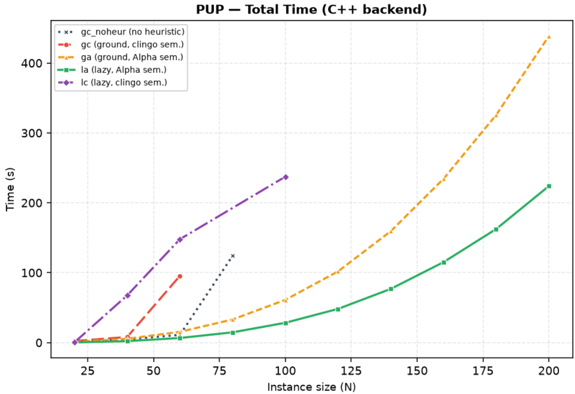
Figure 5.7: Total clingo runtime on PUP across instance sizes for the C++ backend.
