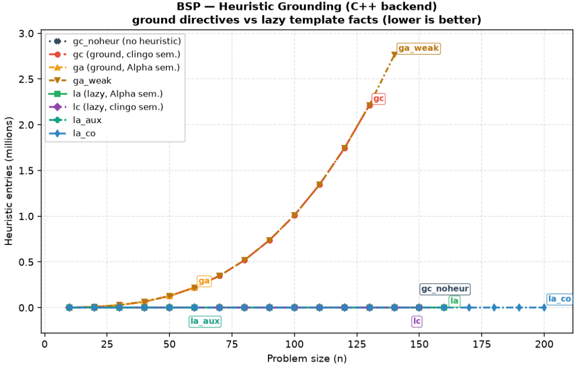
Figure 5.1: Ground heuristic directives against lazy template facts on BSP. The three ground variants coincide by construction, since they unroll the same directive over the same value domain and differ only in the guard that fires it; the four lazy ones and the heuristic-free baseline are indistinguishable from one another at this scale, at two facts and none respectively. Each curve ends at the largest size its variant solves (Table 5.1), so ga stops at n = 60 although the count itself keeps growing.
