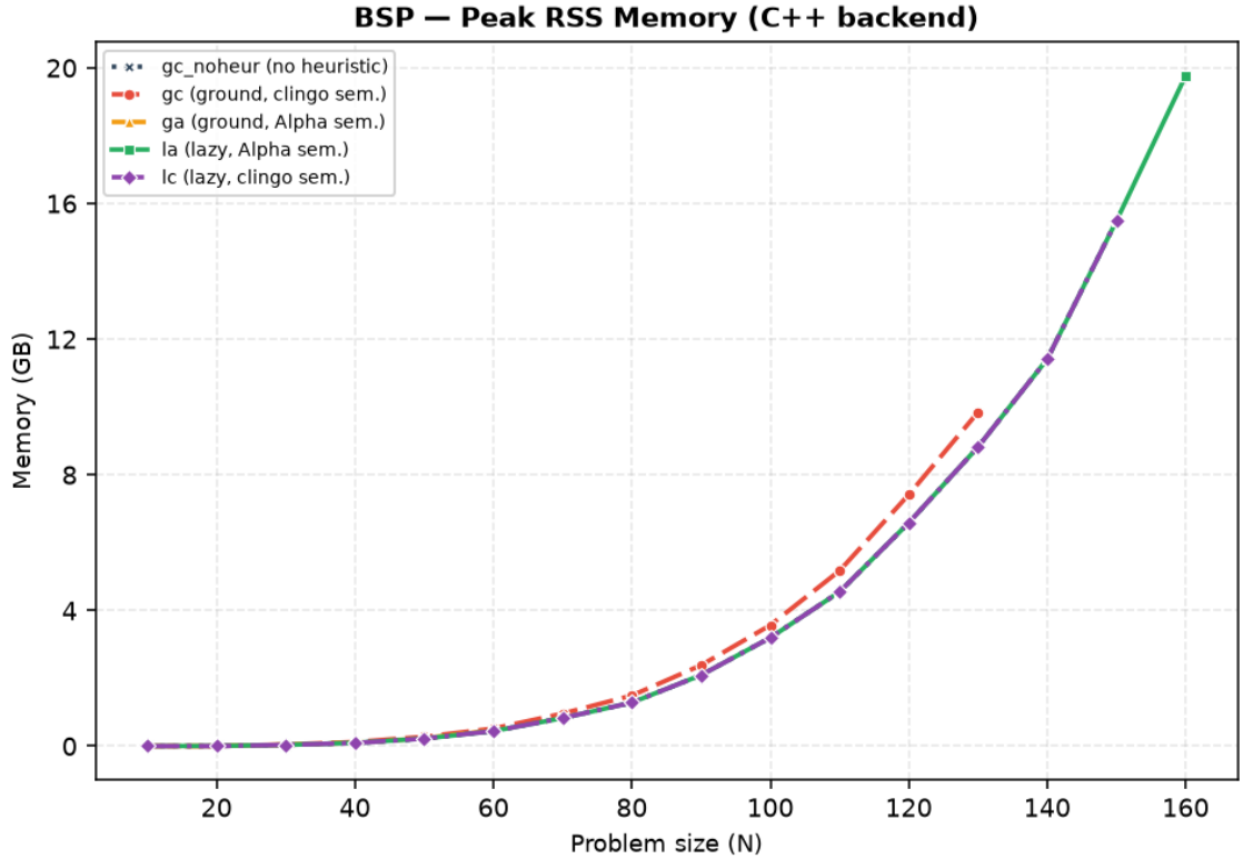
Figure 5.6: BSP: peak resident set size on the C++ backend across instance sizes.
