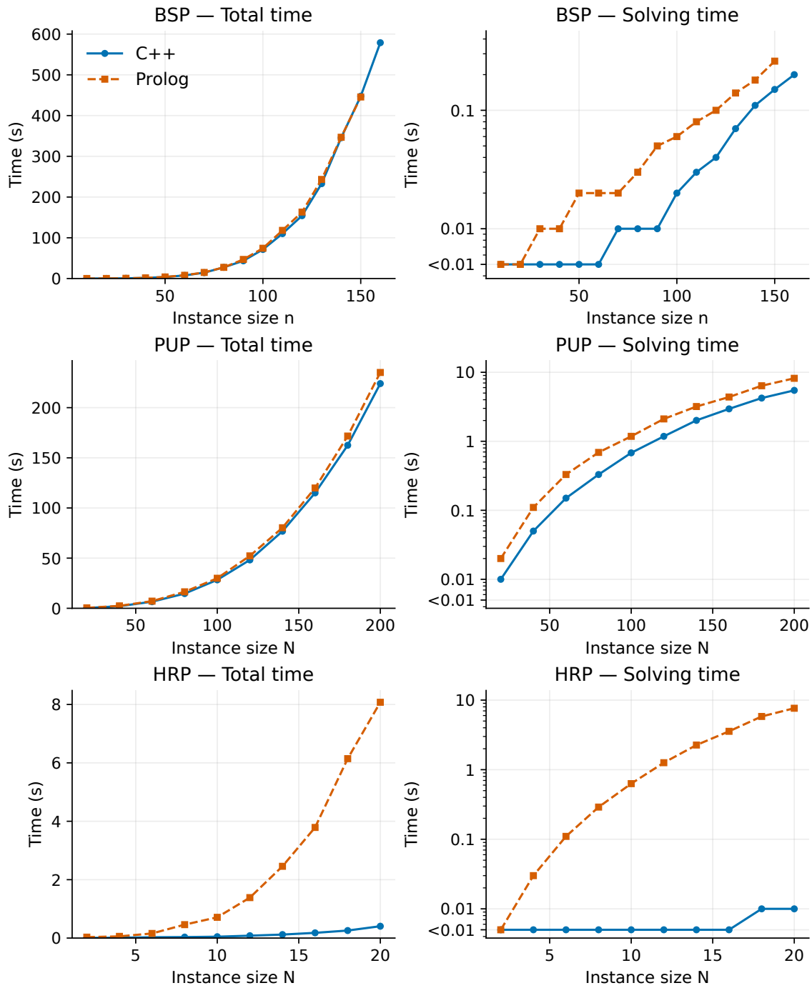
Figure 5.12: The 1a variant on C++ and Prolog across all three families: total clingo time (left) and solving time (right). Each panel has its own vertical scale; the solving panels use a logarithmic scale to keep both backends visible. Only successful runs are plotted, and curves end at the largest solved instance.
