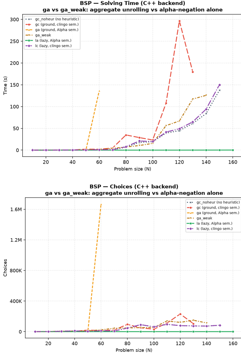
Figure 5.20: Solving time (top) and solver choices (bottom) for BSP comparing the Alpha-like semantics simulations ( ga and ga_weak ) against the baseline variants.
