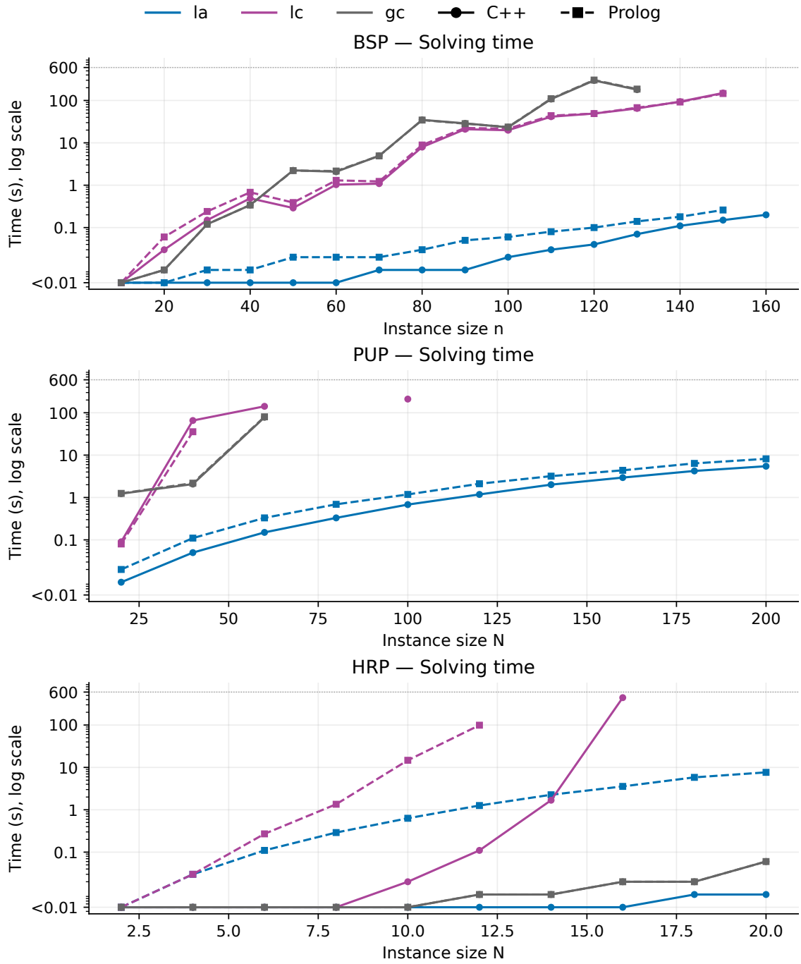
Figure 5.13: Solving time on both backends for 1a, 1c and the ground control gc. Colour identifies the variant; solid circles denote C++ and dashed squares Prolog. Only successful runs are plotted. The dotted line marks 600s for orientation, although the actual budget includes grounding as well. Values reported below 0.01 s are shown at a plotting floor.
