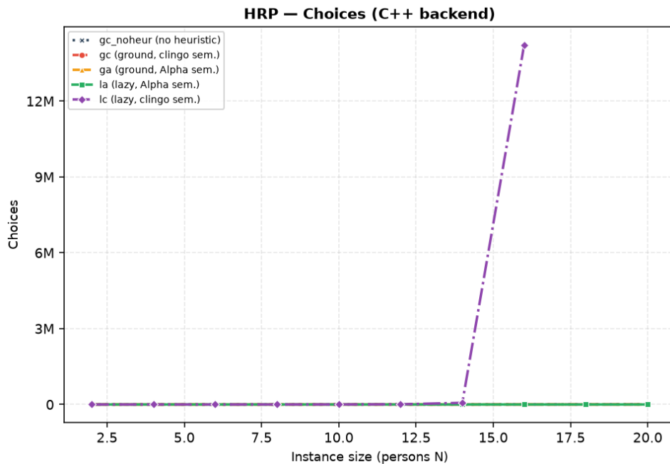
Figure 5.11: HRP: solver choices on the C++ backend. The only diverging curve is lc , analyzed in Section 5.10.
