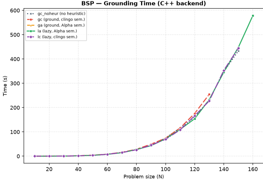
Figure 5.2: Grounding time on BSP for the C++ backend. One run per point; a curve ends where its variant stops solving within the limits.
