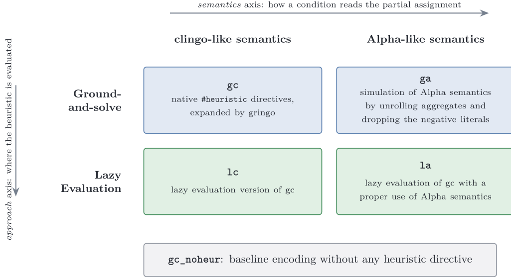
Figure 3.1: The experimental matrix. Prefixes name the approach, suffixes the semantics.
