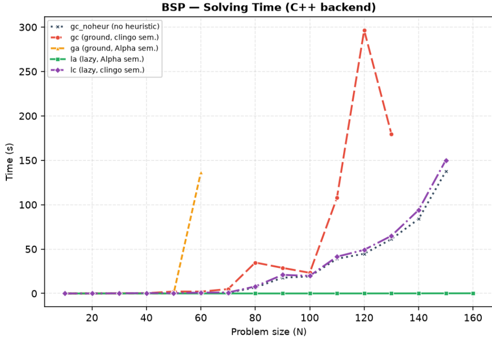
Figure 5.3: Solving time on BSP for the C++ backend, on the same runs as Figure 5.2.
