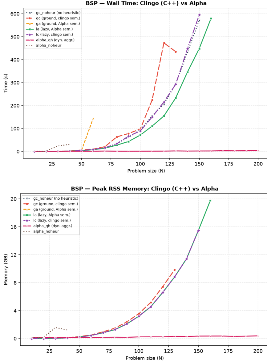
Figure 5.16: BSP benchmark dashboard: the four clingo variants and the heuristic-free baseline gc_noheur compared against Alpha with ( alpha_qh ) and without ( alpha_noheur ) declarative heuristics. Top: total wall-clock time; bottom: peak RSS. Both are runlim external process measures.
