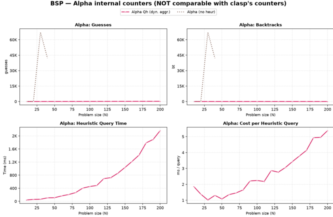
Figure 4.18: BSP internal search counters for Alpha across instance sizes. Top row: with heuristics ( alpha_qh ), guesses remain equal to n with zero backtracks; without heuristics ( alpha_noheur ), search choices explode exponentially. Bottom row: cumulative Prolog query evaluation time for alpha_qh (2.2s total at n = 200 , averaging 1.9 to 5.4 ms per consultation).
