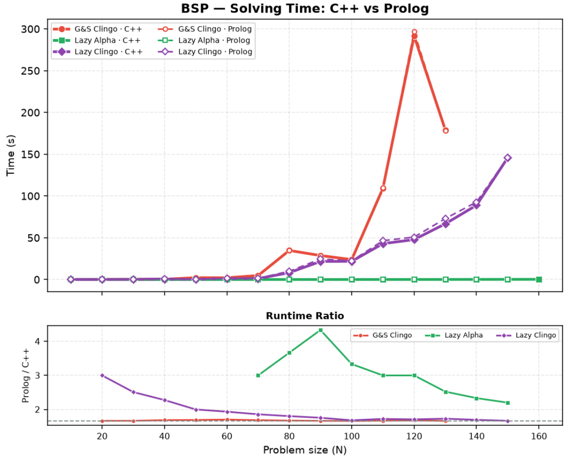
Figure 4.7: BSP: solving time comparison between the two backends. The bottom subplot shows the relative runtime ratio ( \text{Time}_{\text{Prolog}} / \text{Time}_{\text{C++}} ), where values above 1.0 indicate the factor by which the interpreted Prolog backend is slower than compiled C++.
