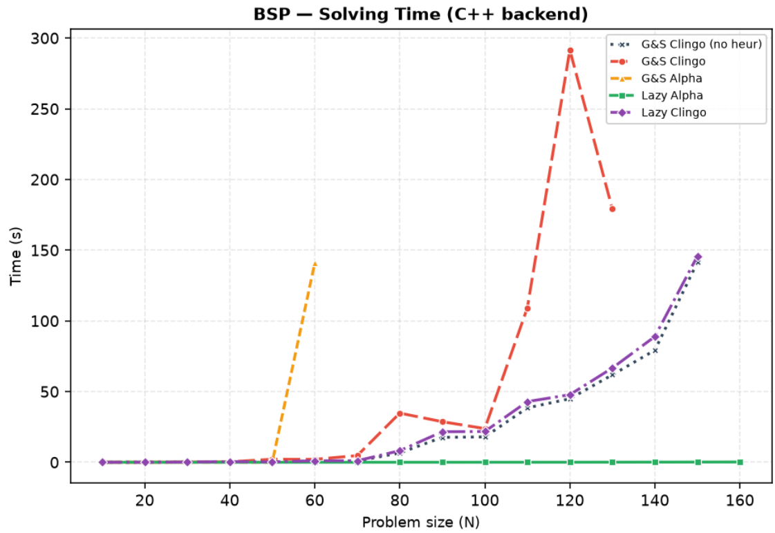
Figure 4.3: la solving time is close to zero across all sizes, whereas ga degrades sharply at n = 60 and times out from n = 70 due to clasp's 16-bit weight saturation ( > 32,767 ).
