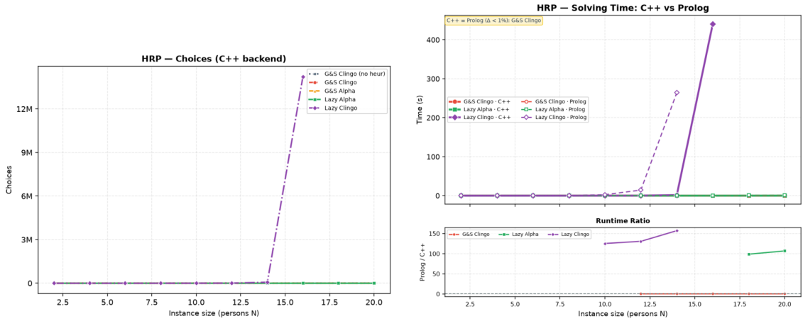
Figure 4.14: HRP: solver choices on the C++ backend (left) and the C++ versus Prolog solving comparison (right). The only diverging curve is 1c, in both plots.
