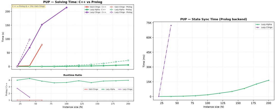
Figure 4.13: PUP: native-versus-Prolog solving comparison (left) and cumulative synchronization cost of the Prolog backend (right). For 1a the synchronization, not the query, is the dominant lazy cost at scale.
