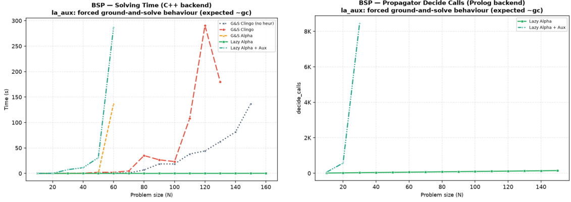
Figure 4.9: BSP, exploratory comparison of the auxiliary form. Left: C++ solving time; la_aux diverges from n = 40 and leaves the chart after n = 60 , while the direct la stays on the axis. Right: propagator decide calls on the Prolog backend; the auxiliary candidates multiply the consultations (573 at n = 20 and 8,452 at n = 30 , against the n calls of the direct form), and the curve ends at n = 30 , the last size the variant solves on that backend.
