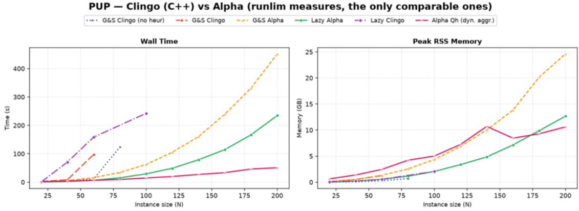
Figure 4.17: PUP: the same comparison. Alpha (no heur ) does not appear because it solves no instance at all, not even double-20 . Here the clingo lazy variant stays within a small factor of Alpha in time and matches it in memory, while the ground simulation ga is worse than Alpha on both axes.
