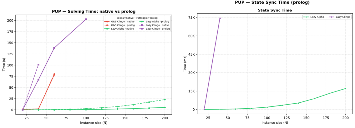
Figure 16: PUP: native-versus-Prolog solving comparison (left) and cumulative synchronization cost of the Prolog backend (right). For 1a the synchronization, not the query, is the dominant lazy cost at scale.
