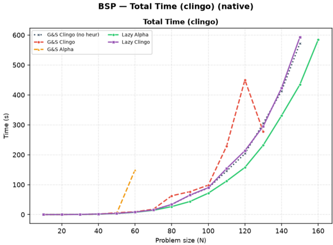
Figure 5: BSP, native backend: total clingo time. Curves are medians over solved instances; a curve ends where its variant stops solving within the limits.
