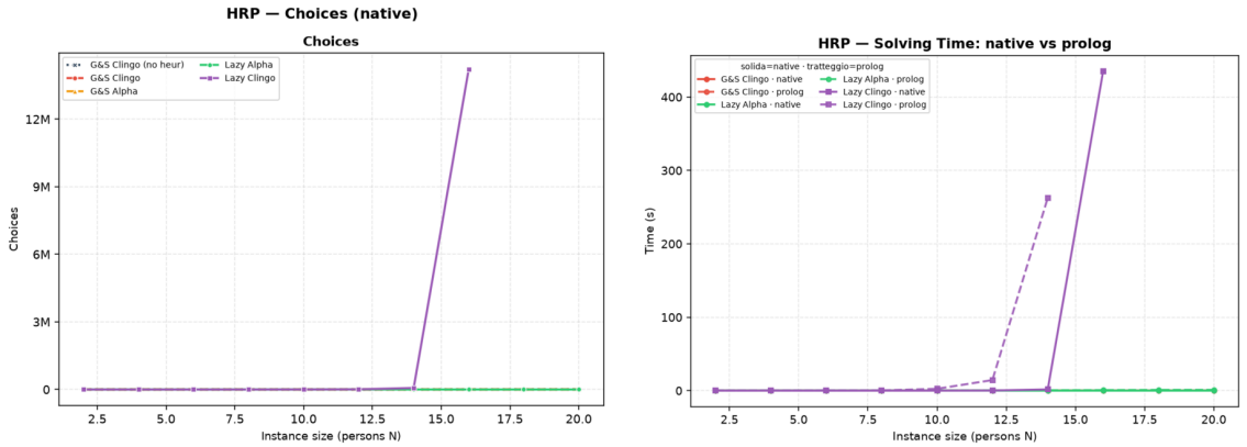
Figure 17: HRP: solver choices on the native backend (left) and the native-versus-Prolog solving comparison (right). The only diverging curve is 1c, in both plots.
