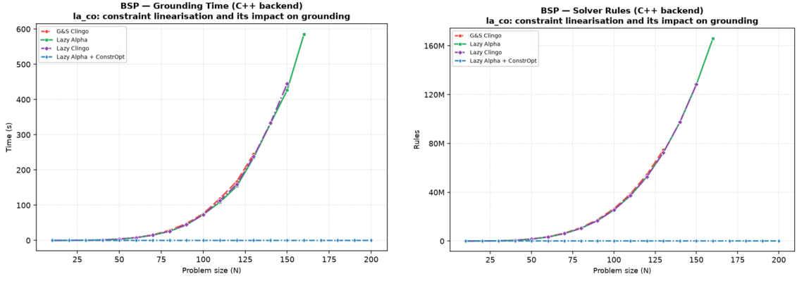
Figure 4.10: BSP, C++ backend, exploratory comparison of the constraint reformulation: grounding time (left) and propositional rules (right). gc , la , and lc overlap because they share the quadratic base encoding (some 52.8 million rules and one to three minutes of grounding at n = 120 ); la_co lies on the horizontal axis of both plots (366 rules, milliseconds of grounding), the visual form of the five-orders-of-magnitude gap discussed in the text.
