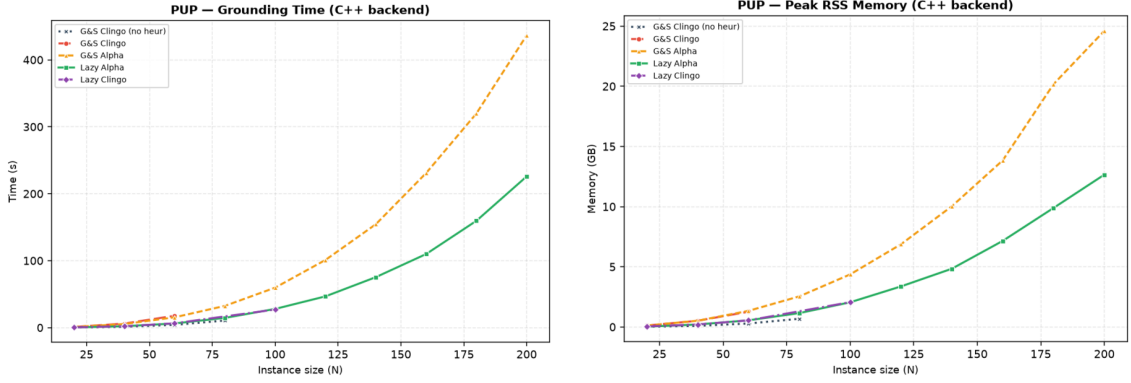
Figure 4.12: PUP, C++ backend: grounding time and peak memory. ga pays the heuristic unrolling (orange) on top of the base growth; la (green) pays the base program only, and stays consistently cheaper at every common size.
