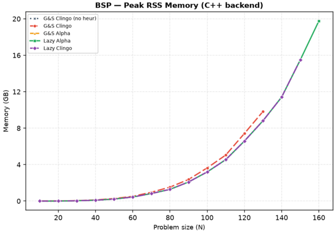
Figure 4.5: BSP, C++ backend: peak resident set size.
