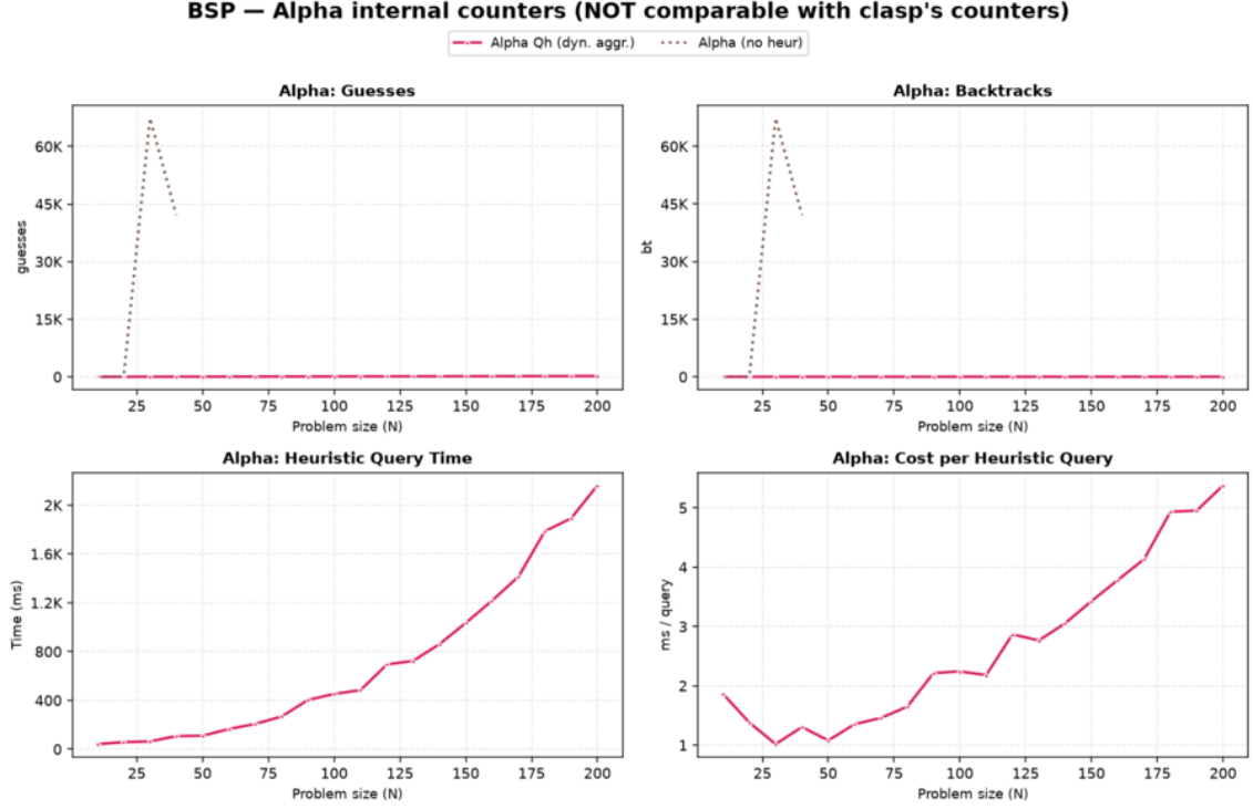
Figure 4.16: BSP, Alpha’s own counters, plotted apart from every clingo measure because they are not commensurable with clasp’s (Section ??). Top row: with the heuristic, guesses stay equal to n and backtracks at zero over the whole range, while the heuristic-free run spikes to some 67,000 of each at n = 30 and stops at n = 40 . Bottom row: the cost of the heuristic itself, which is a Prolog query in this variant — 2.2 seconds cumulative at n = 200 , at 1.9 to 5.4 milliseconds per query.
