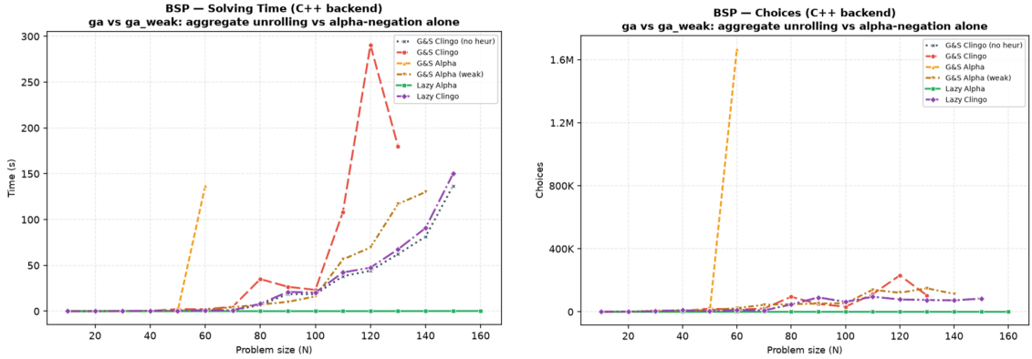
Figure 4.8: BSP, C++ backend, exploratory comparison: solving time (left) and solver choices (right) with both Alpha simulations alongside the main variants. ga is exact up to n = 50 , degrades from n = 51 once its weights leave the representable range, needs 1.7 million choices and 137 seconds of solving at n = 60 , and times out from n = 70 ; ga_weak stays in the baseline’s band over the whole range and reaches n = 140 on both backends, two sizes short of the baseline.
