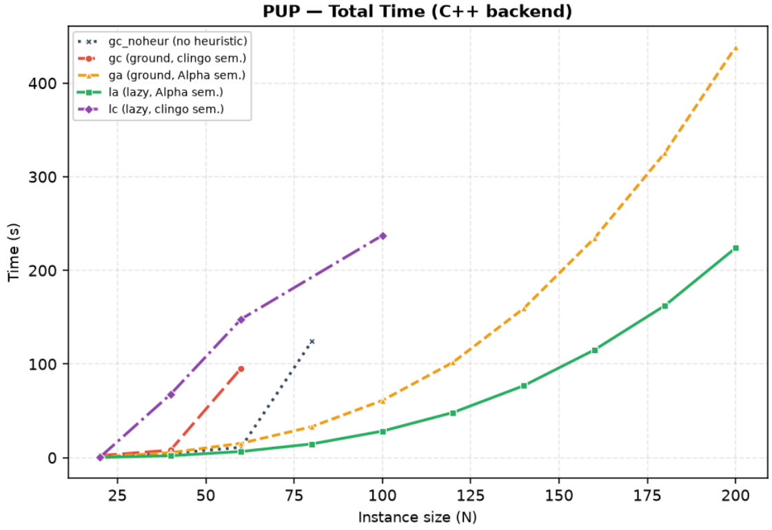
Figure 4.7: Total clingo runtime on PUP across instance sizes for the C++ backend.
