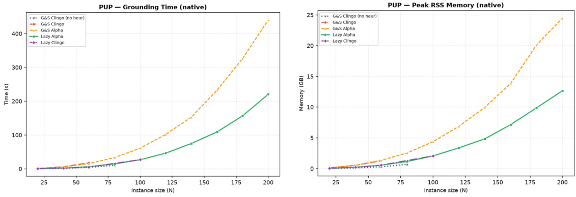
Figure 4.12: PUP, native backend: grounding time and peak memory. ga pays the heuristic unrolling (orange) on top of the base growth; 1a (green) pays the base program only, and stays consistently cheaper at every common size.
