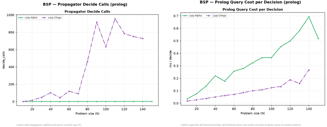
Figure 4.6: BSP, Prolog backend: decide calls and per-decision query cost. The 1c curve pairs tens of thousands of calls with a low unit cost; 1a the opposite.
