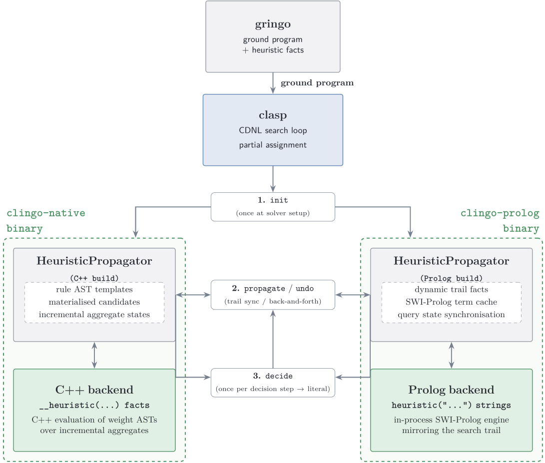
Figure 3: System architecture of the two binary variants ( clingo-native and clingo-prolog ), showing their respective heuristic propagators and evaluation backends attached to clasp.
