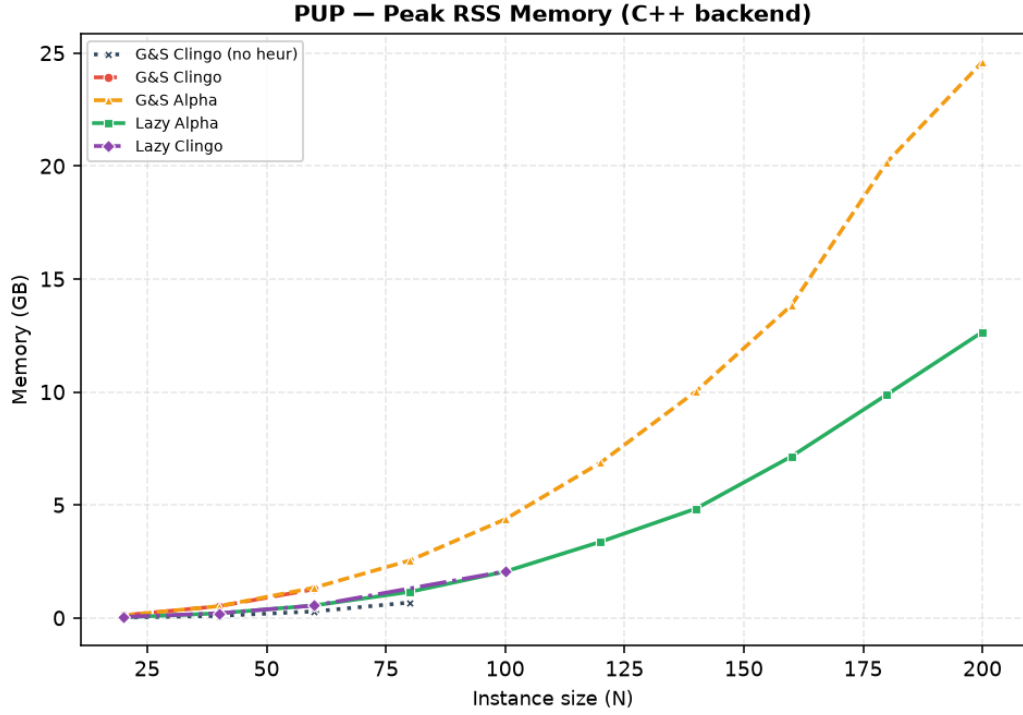
Figure 4.13: Peak memory usage on PUP for the C++ backend, illustrating the 2\times memory reduction of 1a over ga .
