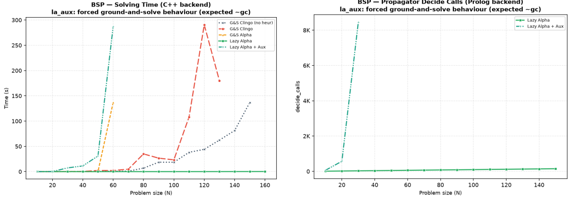
Figure 4.9: Solving time on the C++ backend (left) and number of propagator decide calls on the Prolog backend (right) comparing 1a_aux against direct 1a in BSP.
