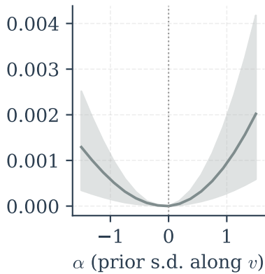
sloppiest direction discrepancy
