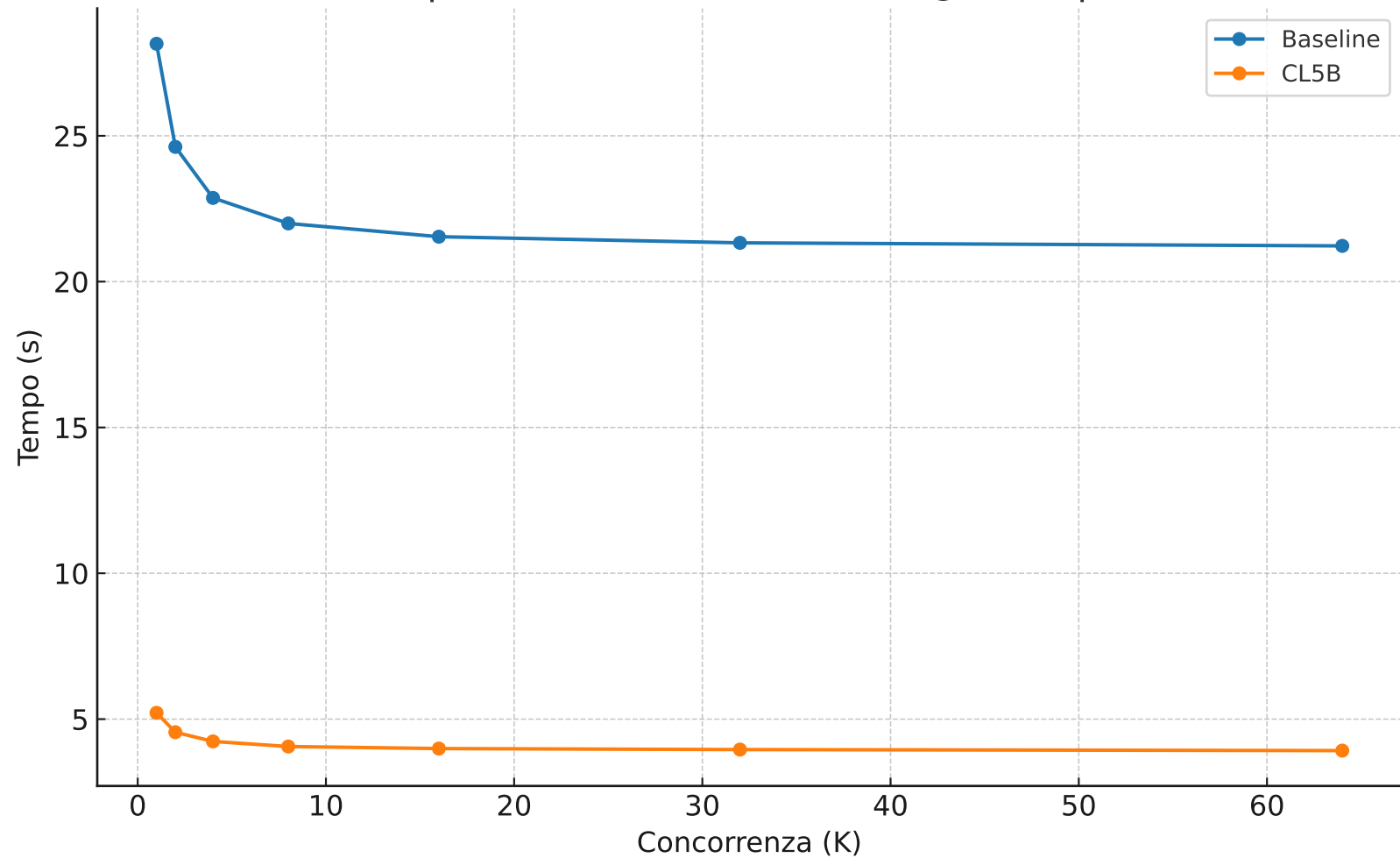
Cap 256.00 KB — RTT 35 ms @20 Mbps
