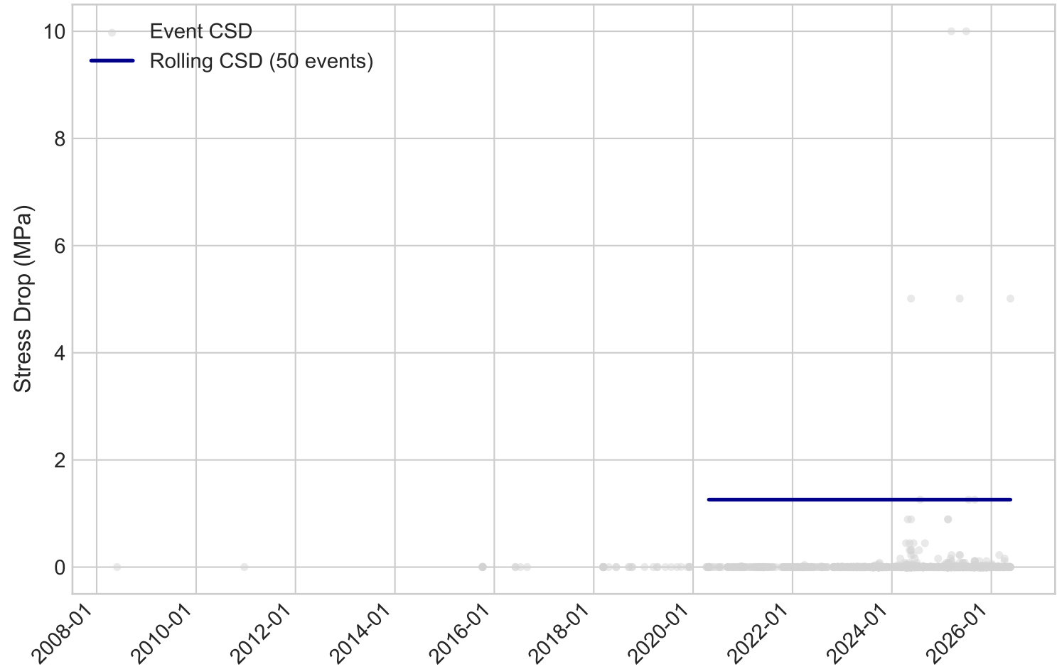
(C) Coulomb Stress Drop (CSD)
