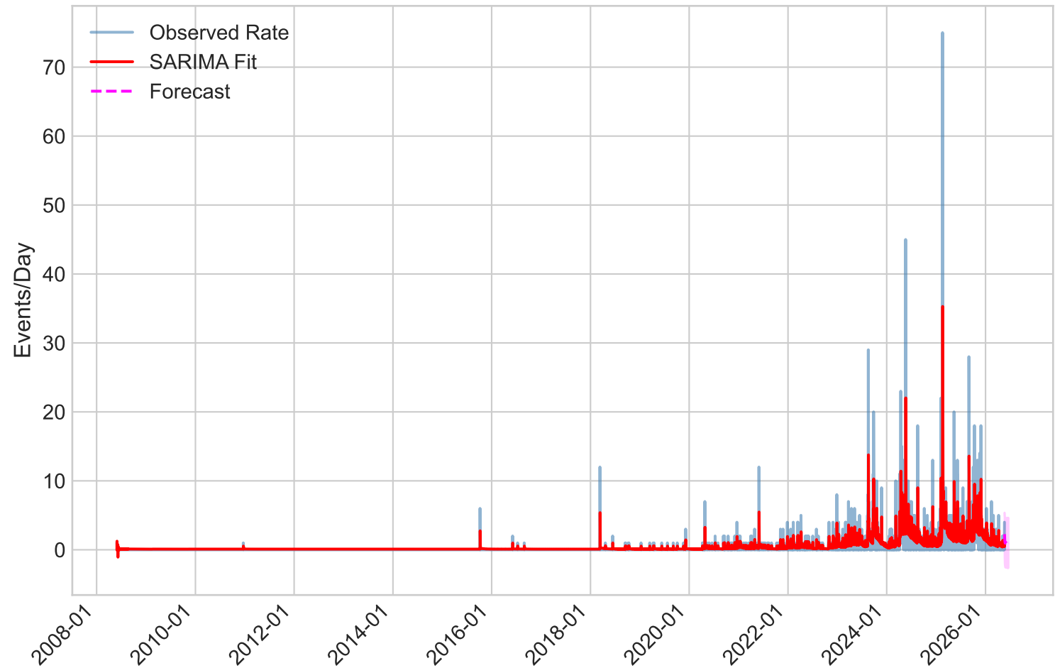
(A) SARIMA Seismic Rate Modeling & Forecast
