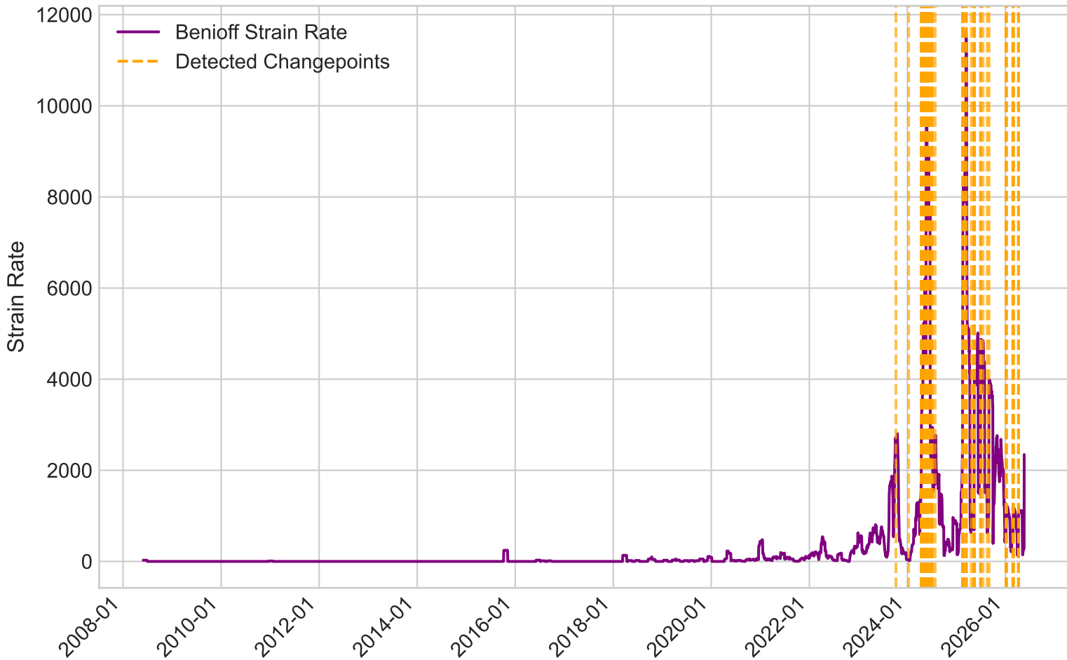
(B) Benioff Strain Release & Structural Changepts
