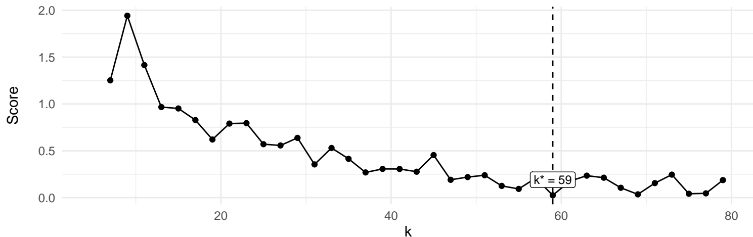
Score combinato (. Diff Moran norm. + . Diff Distanza norm.)
