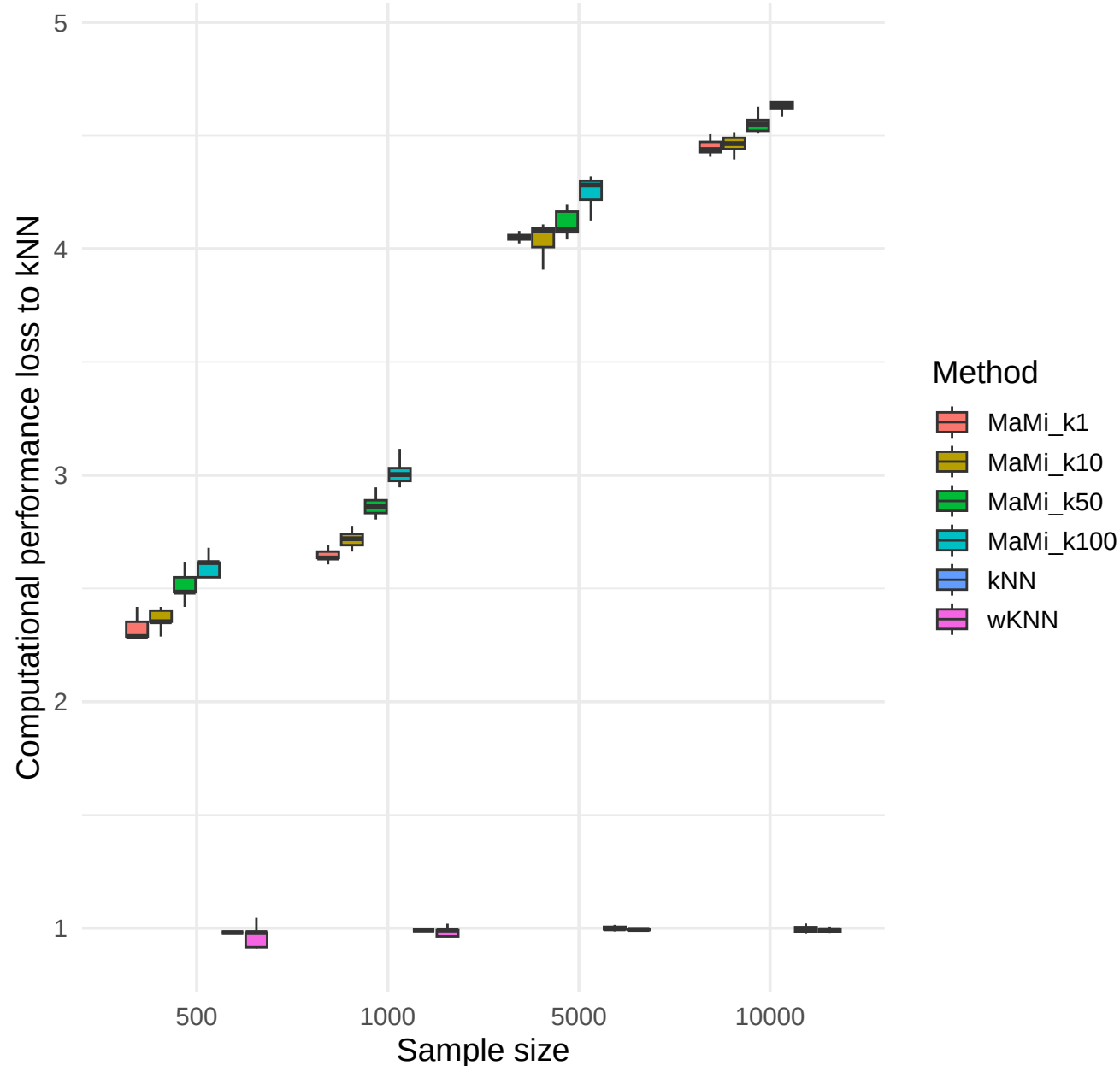
Varying sample size and k2-neighborhood
