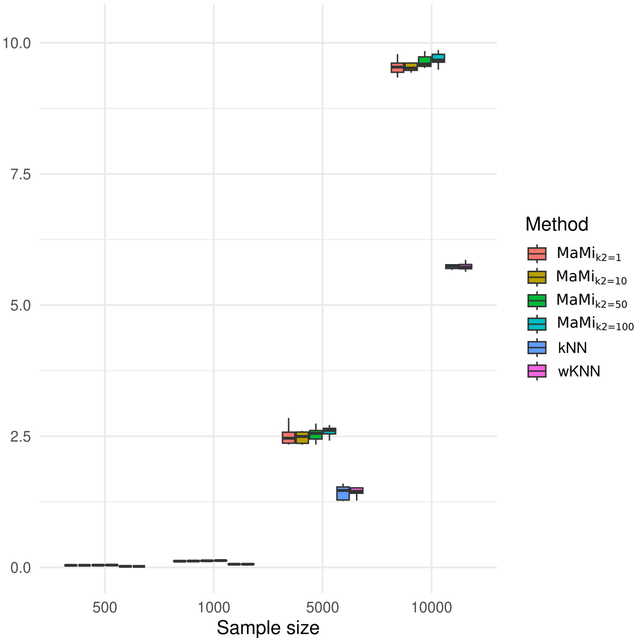
Varying sample size and k2-neighborhood
