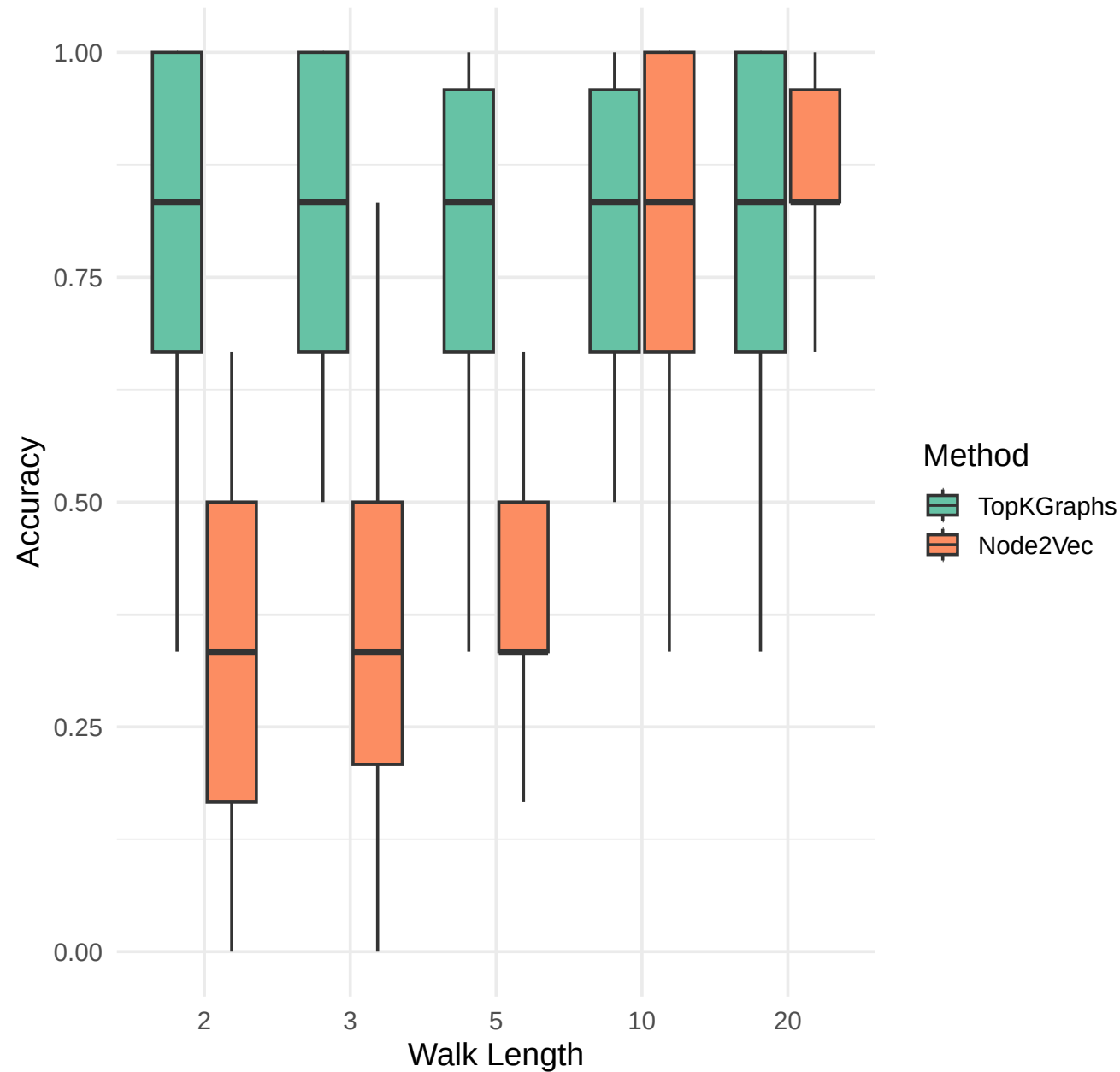
Classification performance
