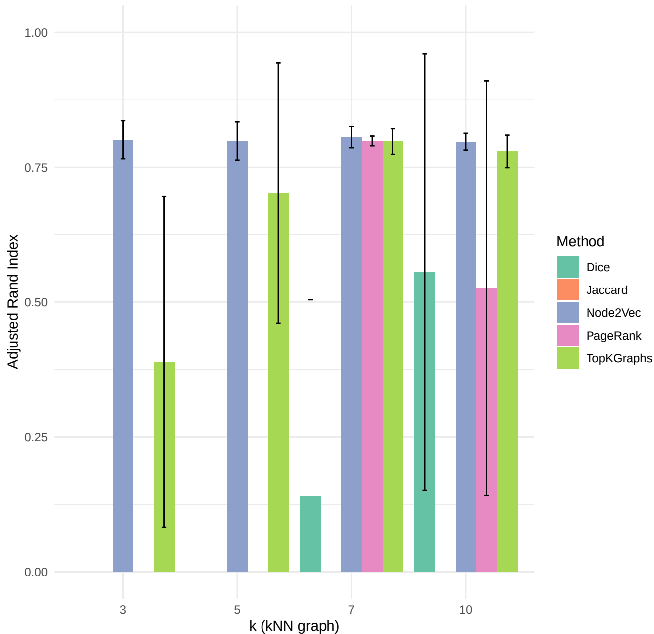
Clustering performance (ARI) across kNN graphs with stability
