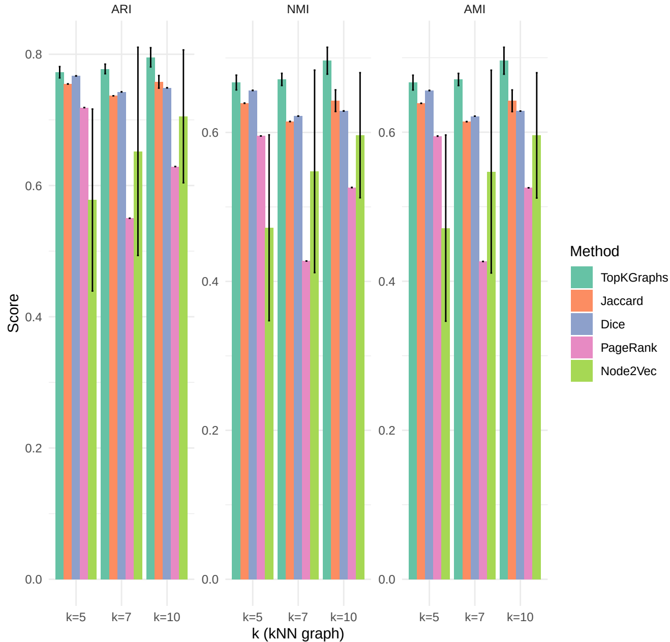
External clustering performance on Iris dataset
