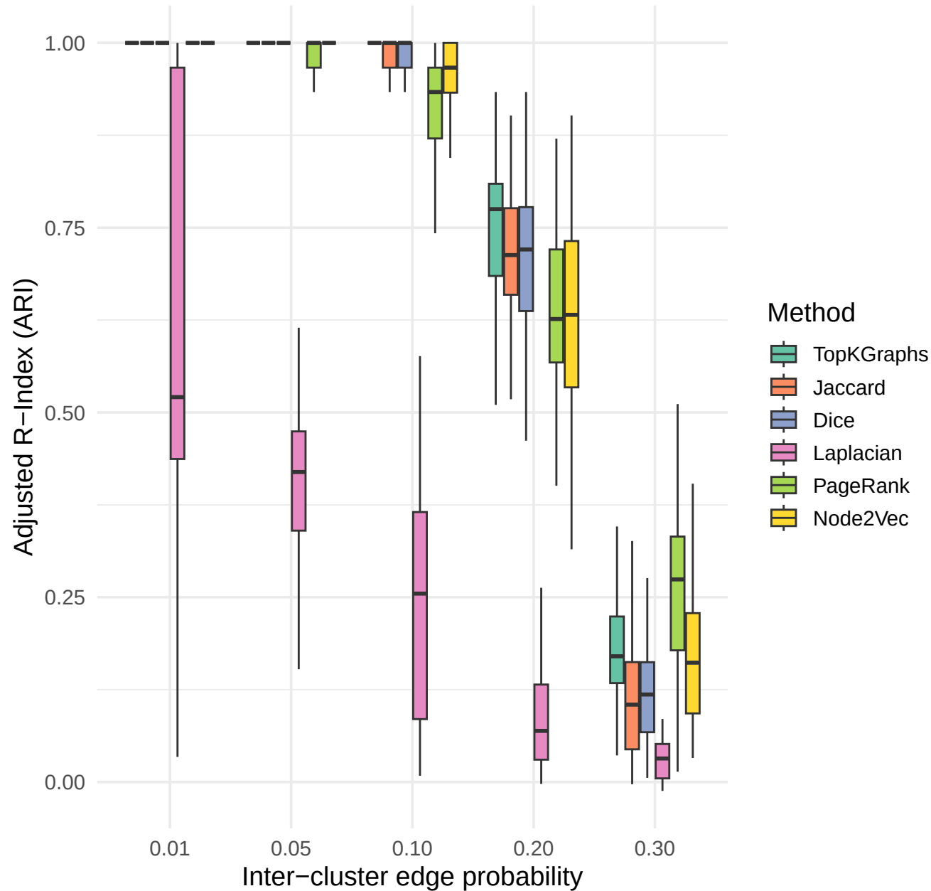
Clustering performance
