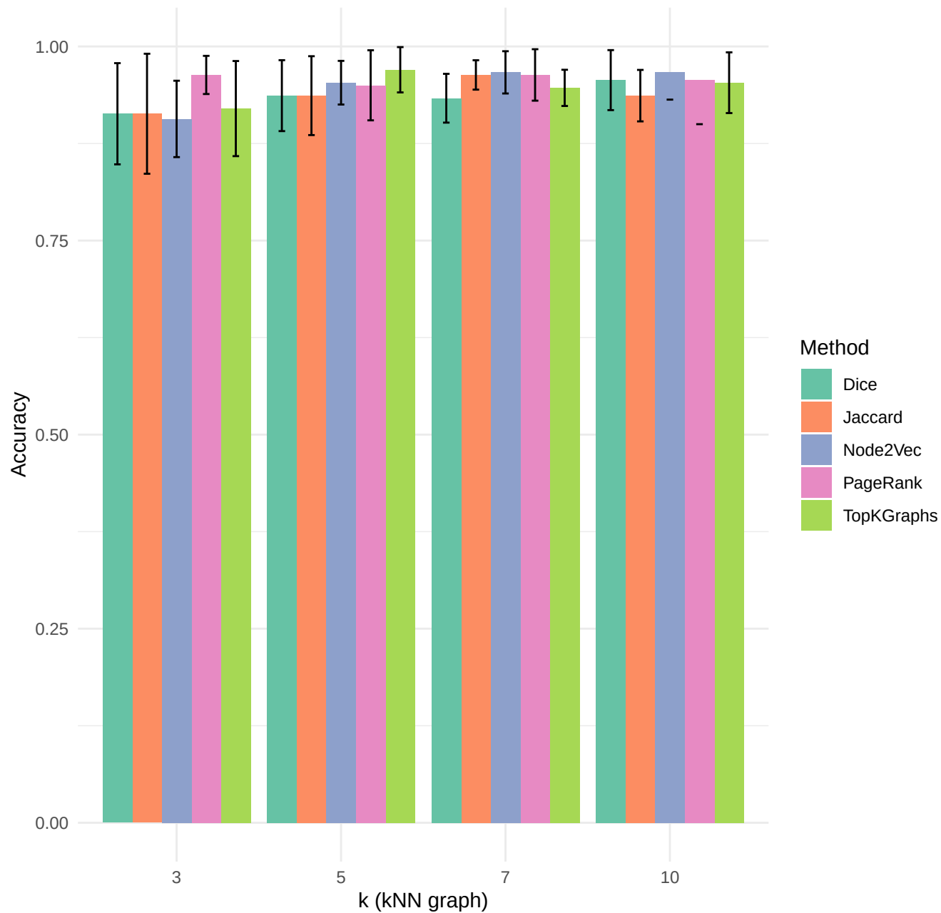
kNN Classification Accuracy (Ecoli)
